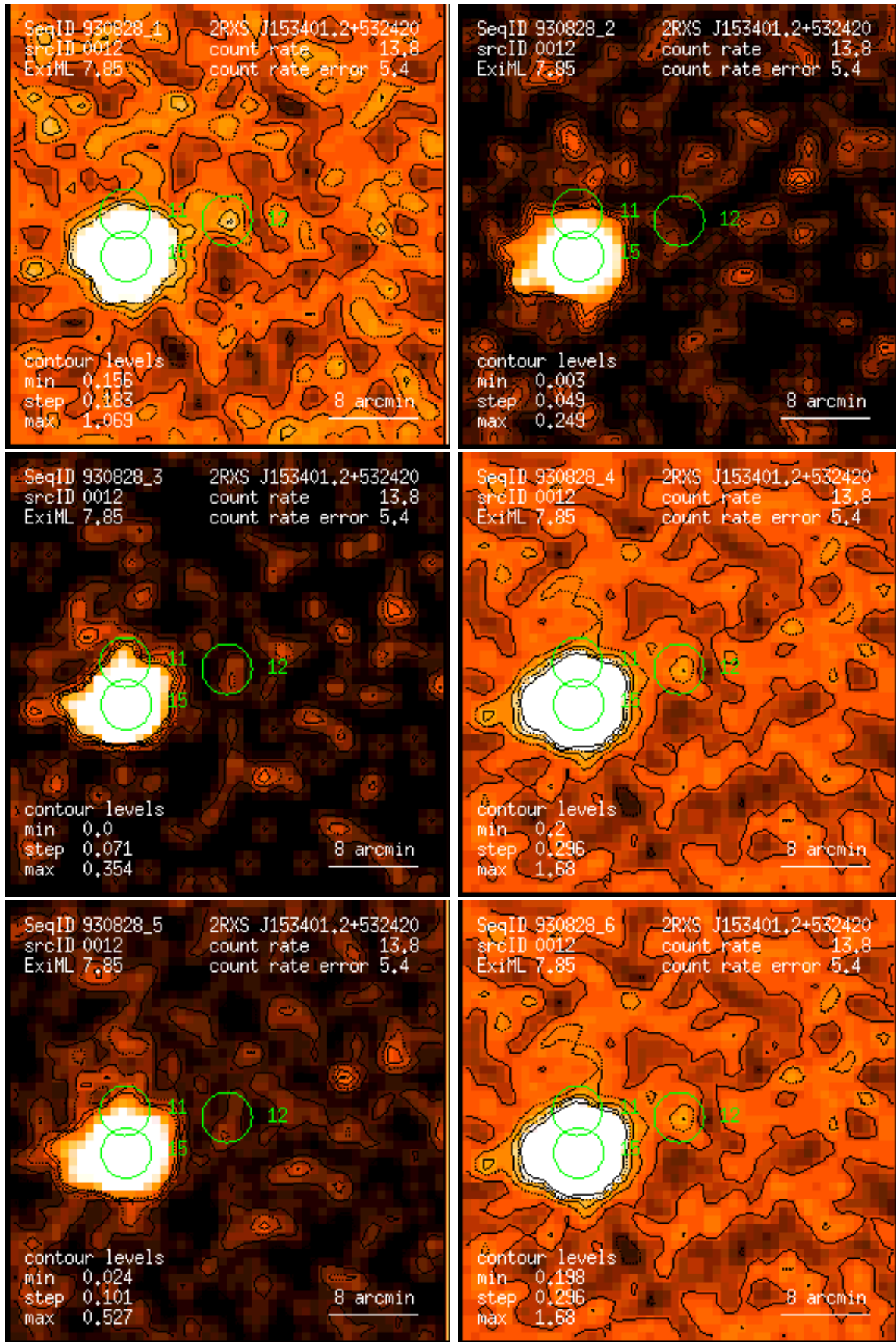
Figure 12: RASS 930828: detection 0012: band rate images, Gaussian filter: (1) PSPC channels 11 – 41, (2) 52 – 90, (3) 91 – 201, (4) 11 – 235, (5) 52 – 201, (6) 11 – 201. Broad band rates in counts/ks. Band rate contour levels in counts/ks/arcmin 2 .
