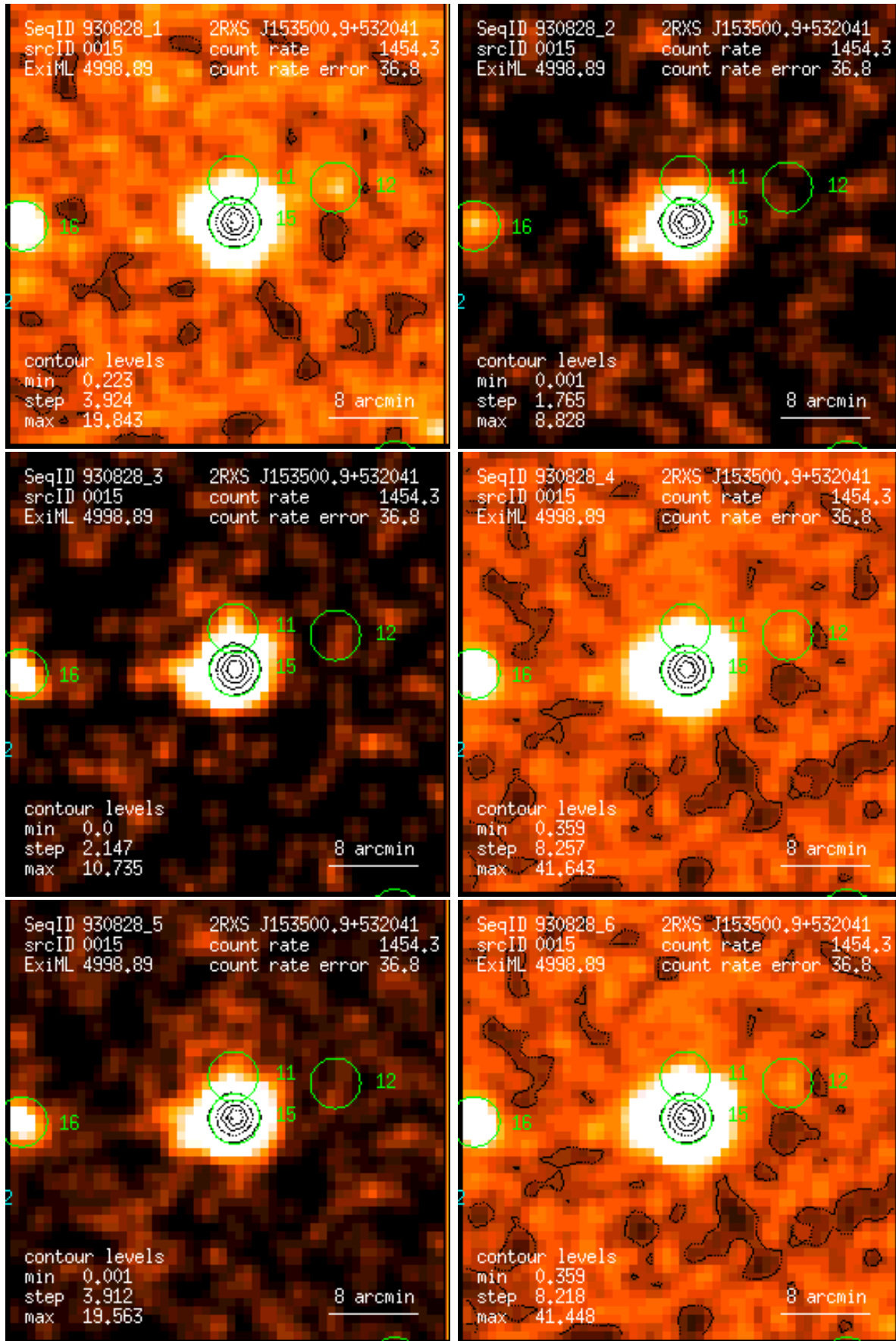
Figure 15: RASS 930828: detection 0015: band rate images, Gaussian filter: (1) PSPC channels 11 – 41, (2) 52 – 90, (3) 91 – 201, (4) 11 – 235, (5) 52 – 201, (6) 11 – 201. Broad band rates in counts/ks. Band rate contour levels in counts/ks/arcmin 2 .
