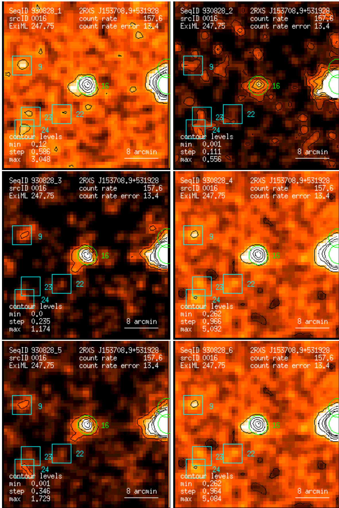
Figure 16: RASS 930828: detection 0016: band rate images, Gaussian filter: (1) PSPC channels 11 – 41, (2) 52 – 90, (3) 91 – 201, (4) 11 – 235, (5) 52 – 201, (6) 11 – 201. Broad band rates in counts/ks. Band rate contour levels in counts/ks/arcmin 2 .
