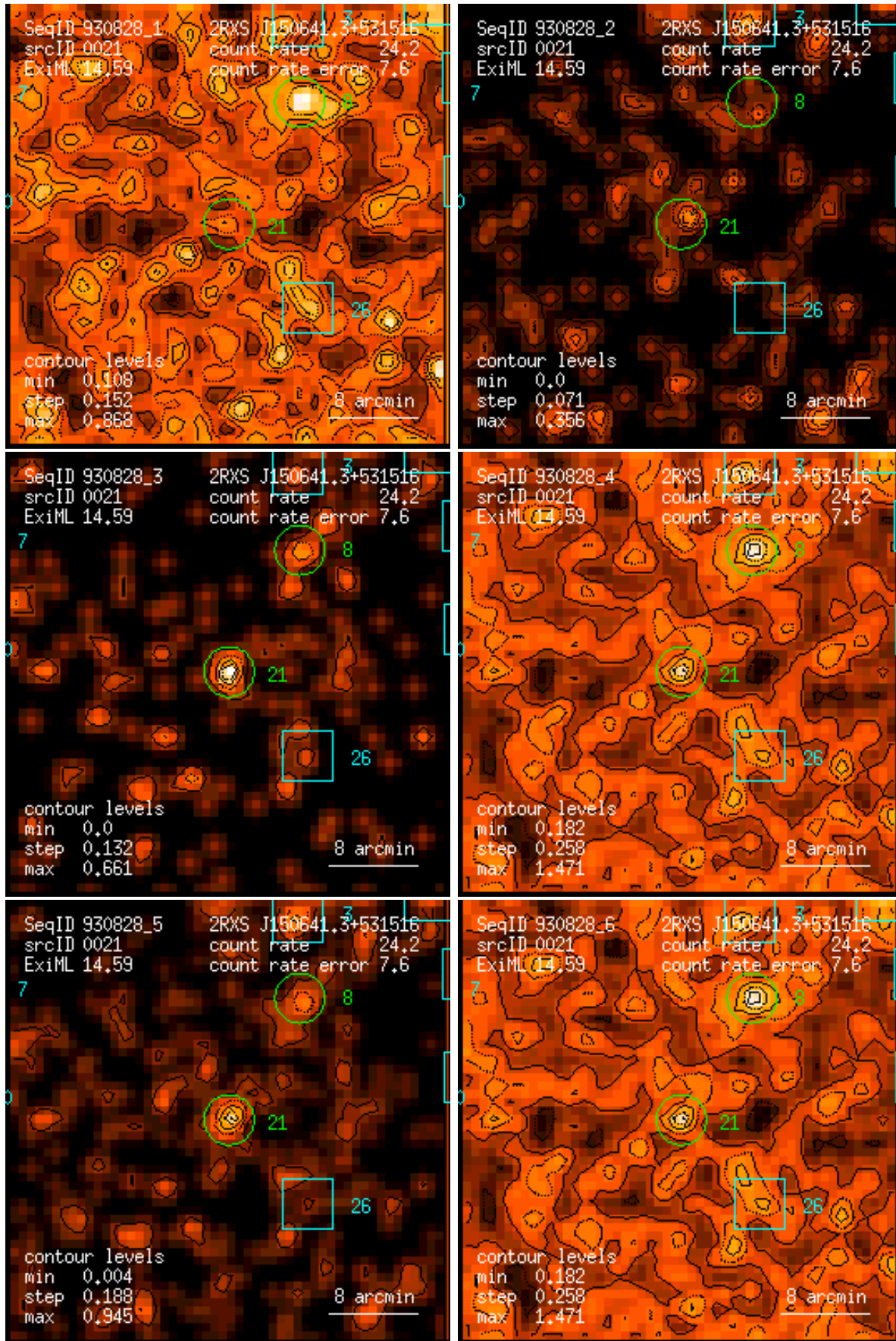
Figure 21: RASS 930828: detection 0021: band rate images, Gaussian filter: (1) PSPC channels 11 – 41, (2) 52 – 90, (3) 91 – 201, (4) 11 – 235, (5) 52 – 201, (6) 11 – 201. Broad band rates in counts/ks. Band rate contour levels in counts/ks/arcmin 2 .
