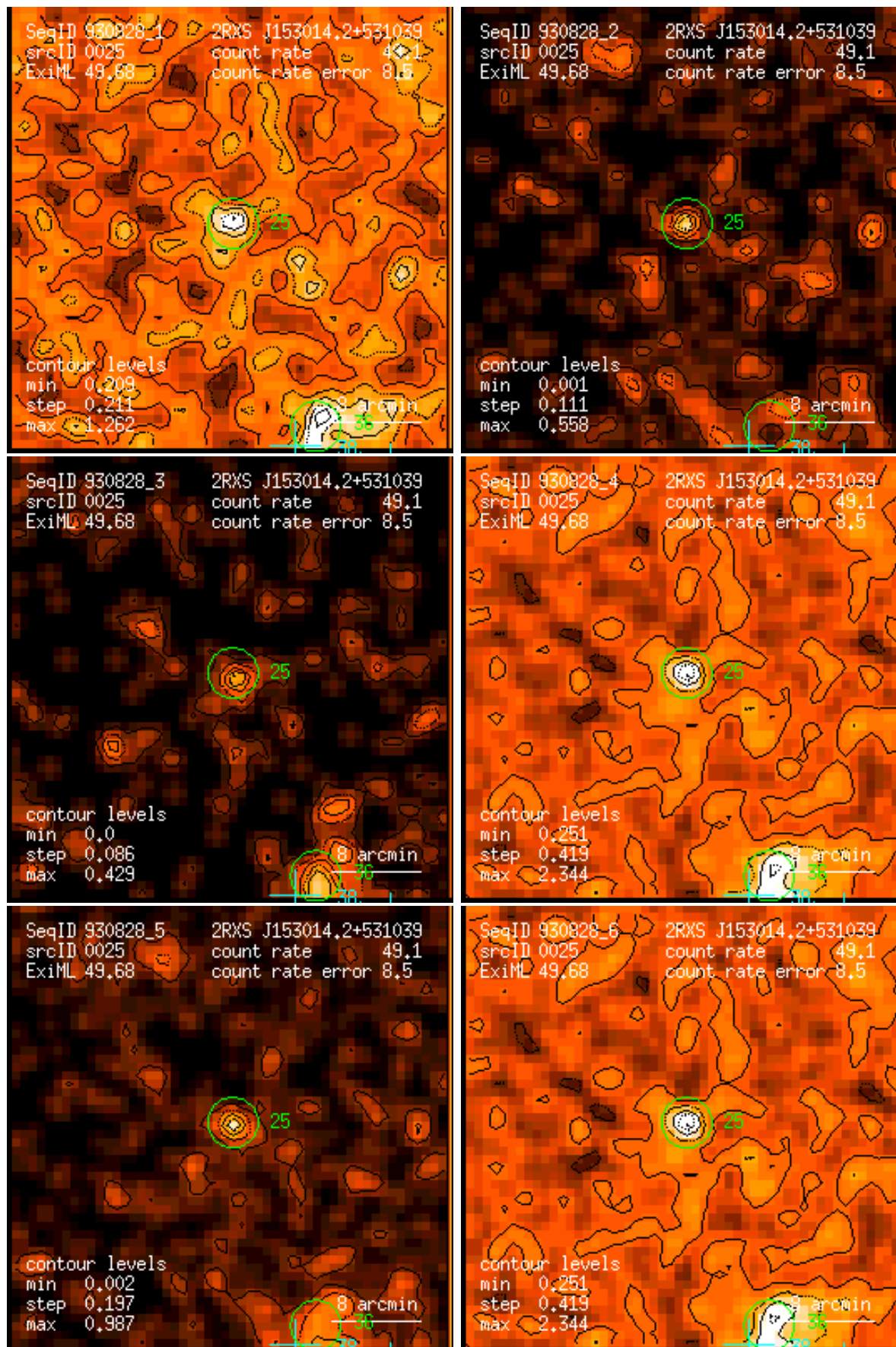
Figure 25: RASS 930828: detection 0025: band rate images, Gaussian filter: (1) PSPC channels 11 – 41, (2) 52 – 90, (3) 91 – 201, (4) 11 – 235, (5) 52 – 201, (6) 11 – 201. Broad band rates in counts/ks. Band rate contour levels in counts/ks/arcmin 2 .
