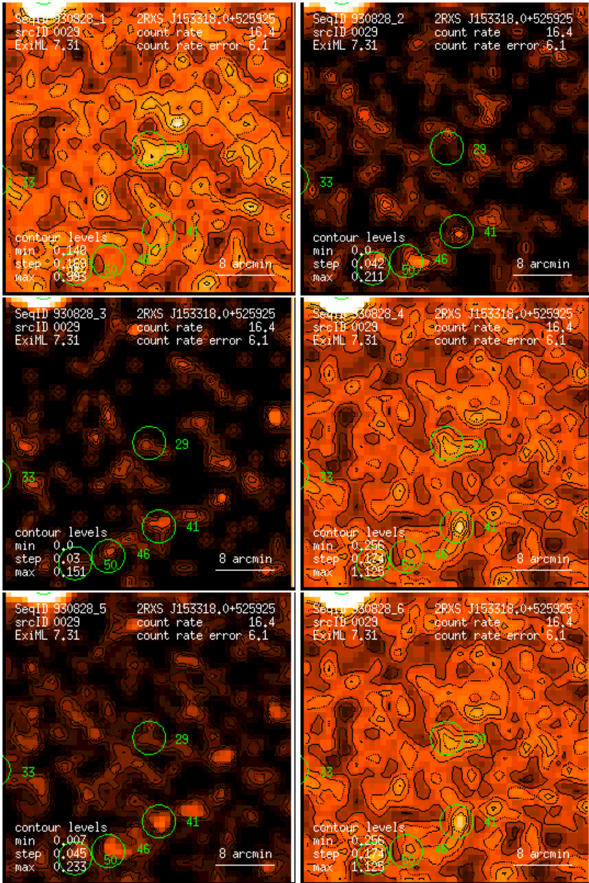
Figure 29: RASS 930828: detection 0029: band rate images, Gaussian filter: (1) PSPC channels 11 – 41, (2) 52 – 90, (3) 91 – 201, (4) 11 – 235, (5) 52 – 201, (6) 11 – 201. Broad band rates in counts/ks. Band rate contour levels in counts/ks/arcmin 2 .
