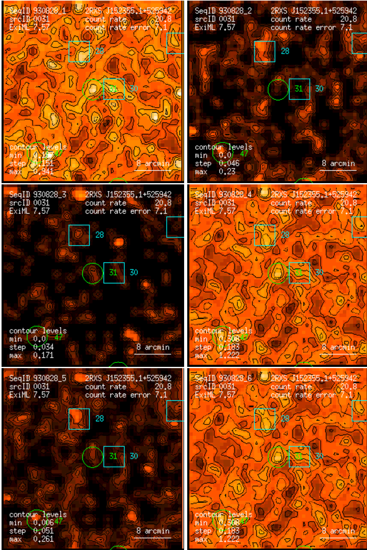
Figure 31: RASS 930828: detection 0031: band rate images, Gaussian filter: (1) PSPC channels 11 – 41, (2) 52 – 90, (3) 91 – 201, (4) 11 – 235, (5) 52 – 201, (6) 11 – 201. Broad band rates in counts/ks. Band rate contour levels in counts/ks/arcmin 2 .
