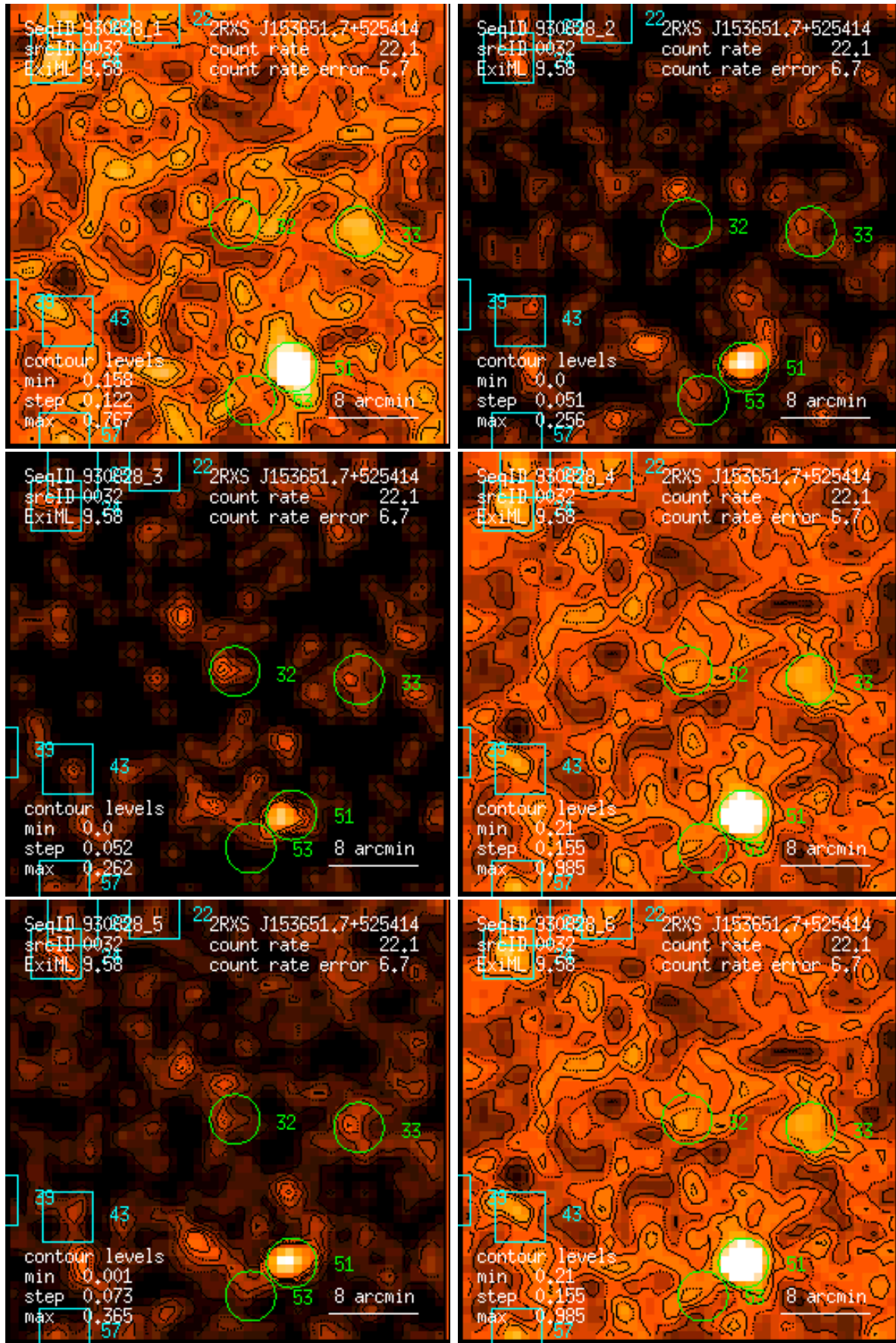
Figure 32: RASS 930828: detection 0032: band rate images, Gaussian filter: (1) PSPC channels 11 – 41, (2) 52 – 90, (3) 91 – 201, (4) 11 – 235, (5) 52 – 201, (6) 11 – 201. Broad band rates in counts/ks. Band rate contour levels in counts/ks/arcmin 2 .
