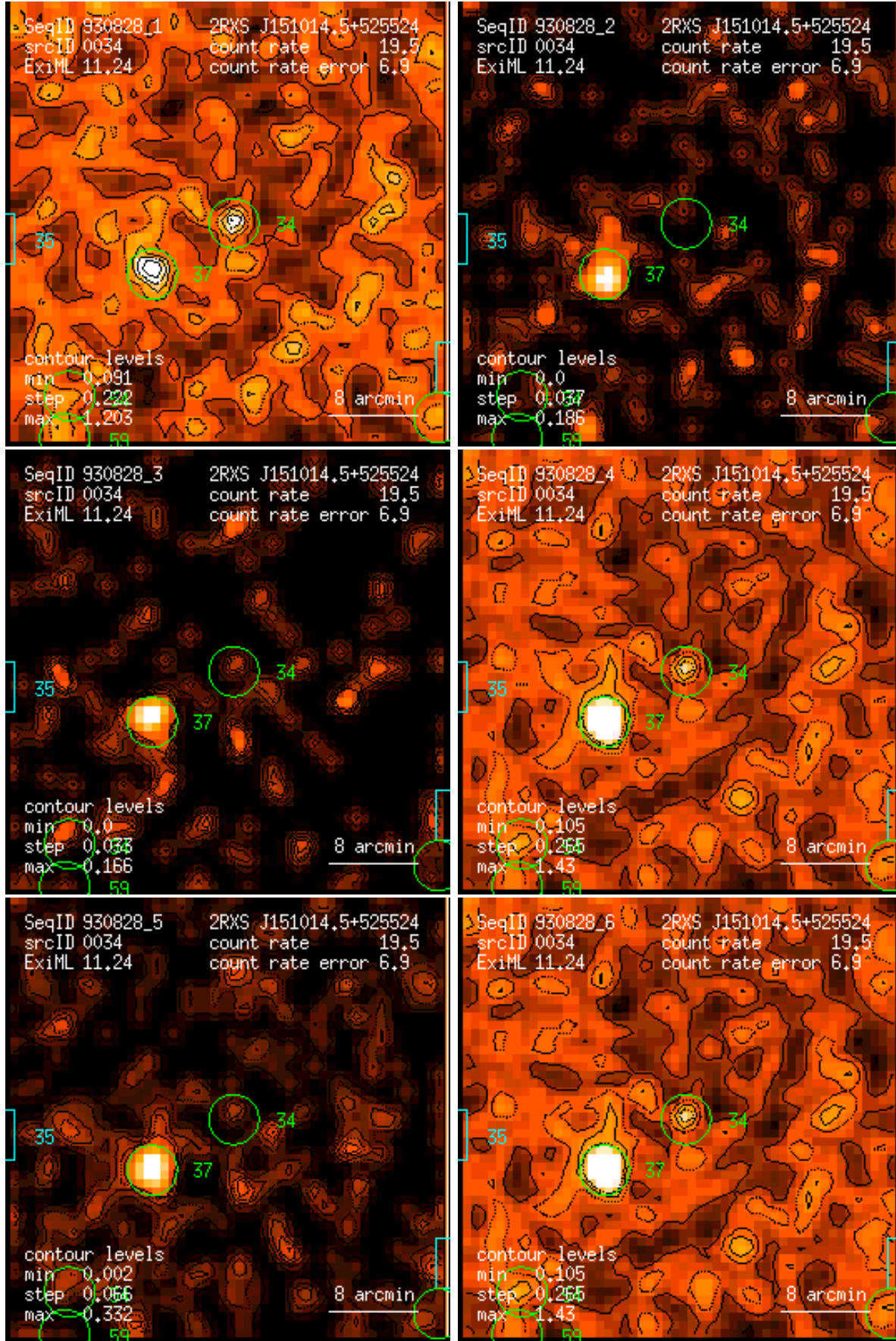
Figure 34: RASS 930828: detection 0034: band rate images, Gaussian filter: (1) PSPC channels 11 – 41, (2) 52 – 90, (3) 91 – 201, (4) 11 – 235, (5) 52 – 201, (6) 11 – 201. Broad band rates in counts/ks. Band rate contour levels in counts/ks/arcmin 2 .
