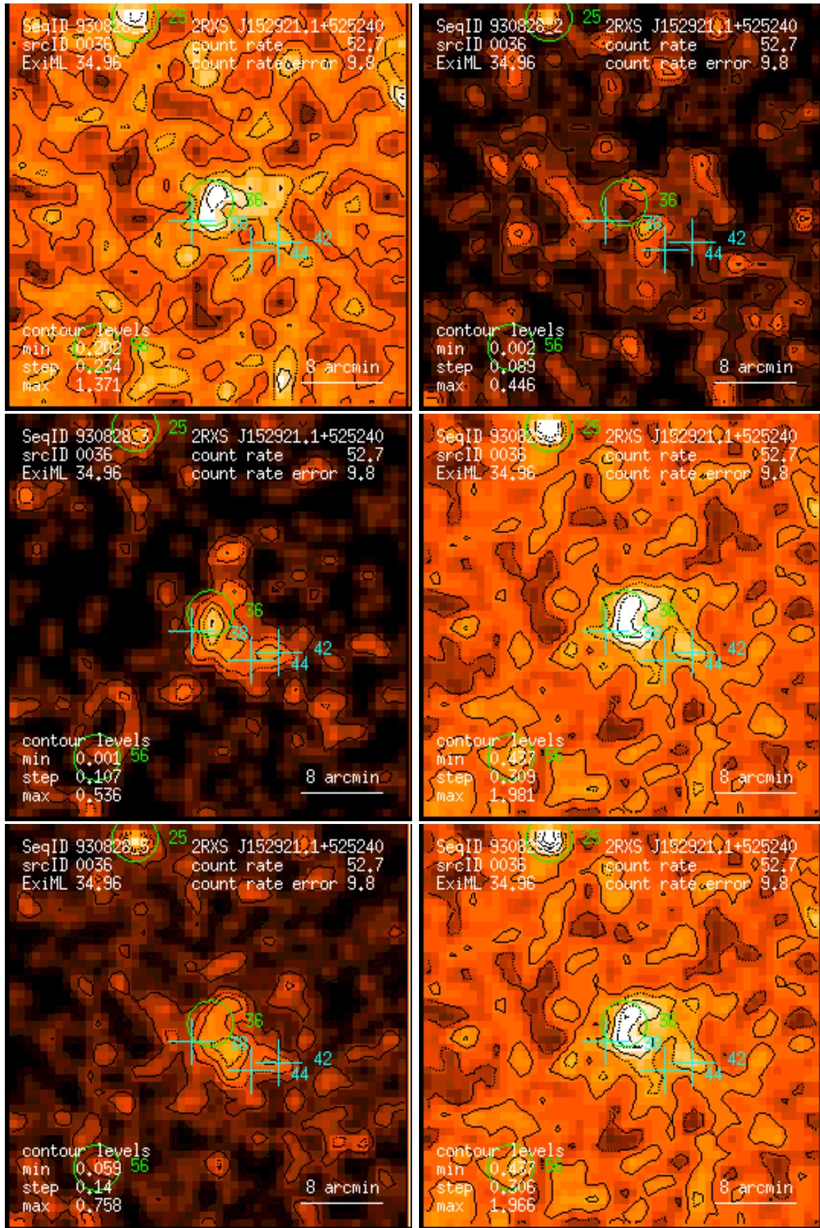
Figure 36: RASS 930828: detection 0036: band rate images, Gaussian filter: (1) PSPC channels 11 – 41, (2) 52 – 90, (3) 91 – 201, (4) 11 – 235, (5) 52 – 201, (6) 11 – 201. Broad band rates in counts/ks. Band rate contour levels in counts/ks/arcmin 2 .
