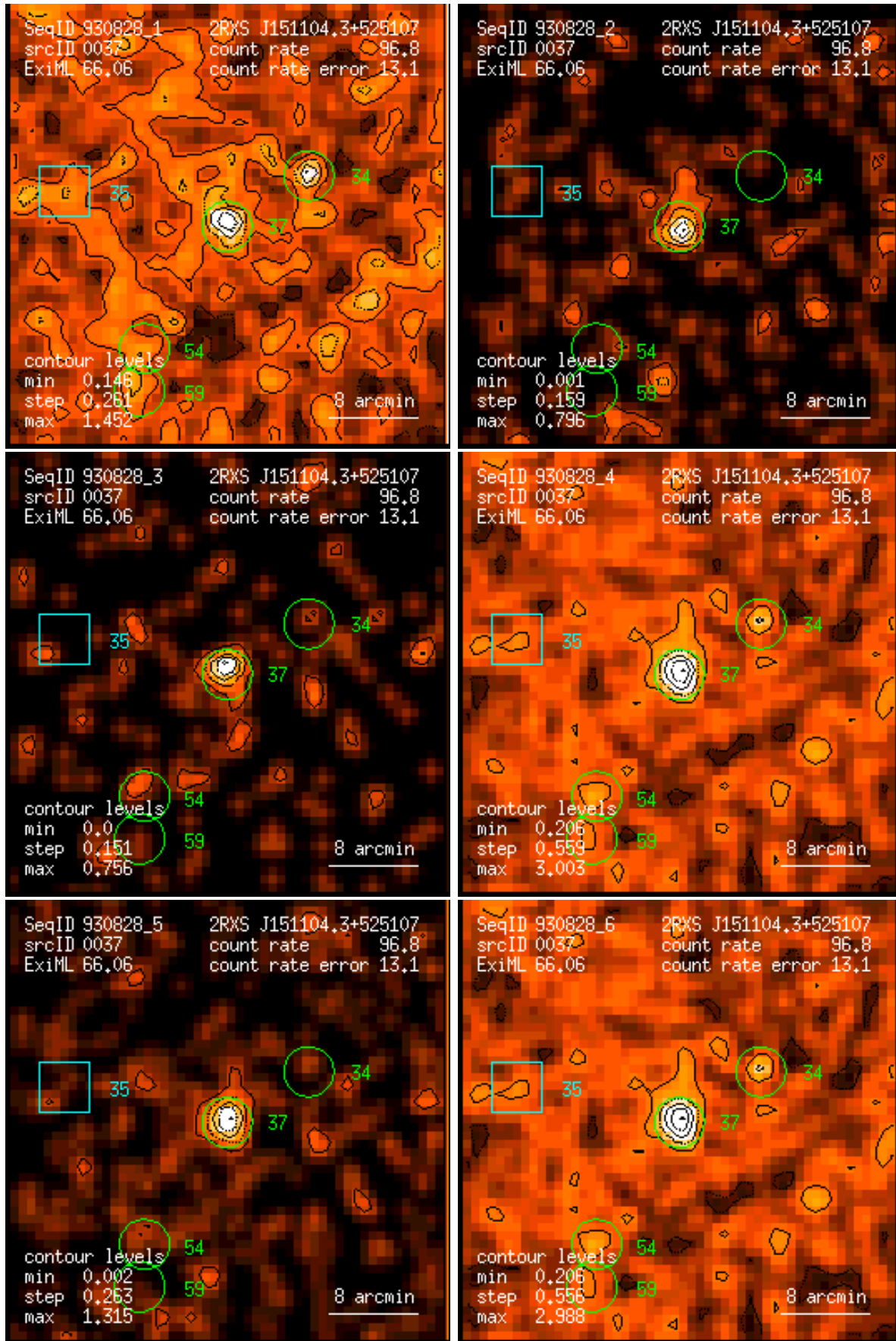
Figure 37: RASS 930828: detection 0037: band rate images, Gaussian filter: (1) PSPC channels 11 – 41, (2) 52 – 90, (3) 91 – 201, (4) 11 – 235, (5) 52 – 201, (6) 11 – 201. Broad band rates in counts/ks. Band rate contour levels in counts/ks/arcmin 2 .
