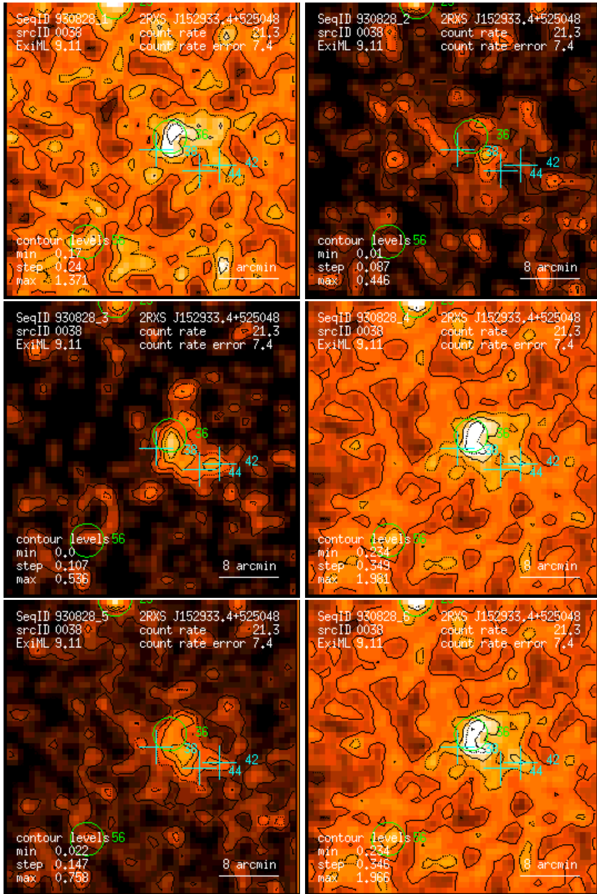
Figure 38: RASS 930828: detection 0038: band rate images, Gaussian filter: (1) PSPC channels 11 – 41, (2) 52 – 90, (3) 91 – 201, (4) 11 – 235, (5) 52 – 201, (6) 11 – 201. Broad band rates in counts/ks. Band rate contour levels in counts/ks/arcmin 2 .
