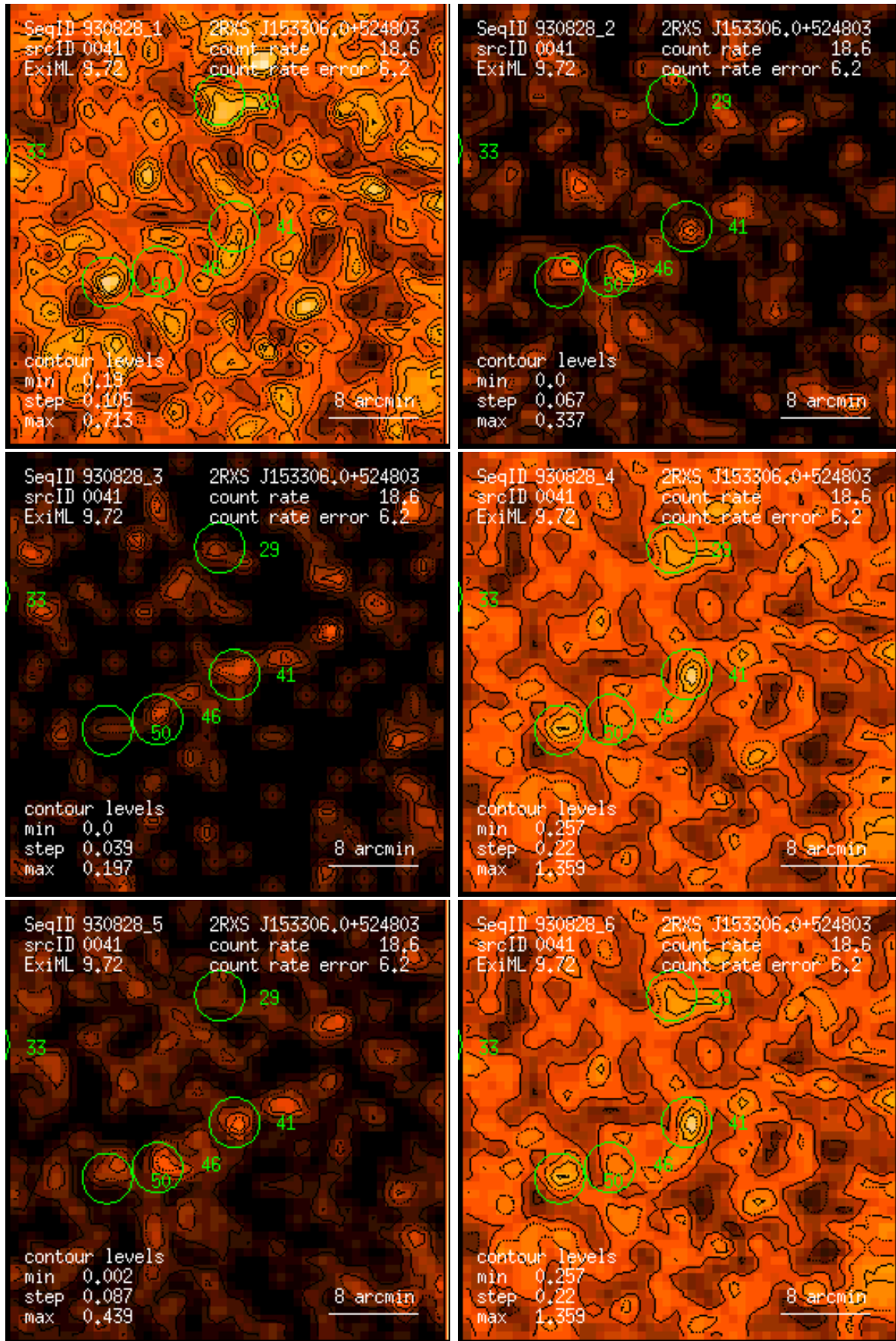
Figure 41: RASS 930828: detection 0041: band rate images, Gaussian filter: (1) PSPC channels 11 – 41, (2) 52 – 90, (3) 91 – 201, (4) 11 – 235, (5) 52 – 201, (6) 11 – 201. Broad band rates in counts/ks. Band rate contour levels in counts/ks/arcmin 2 .
