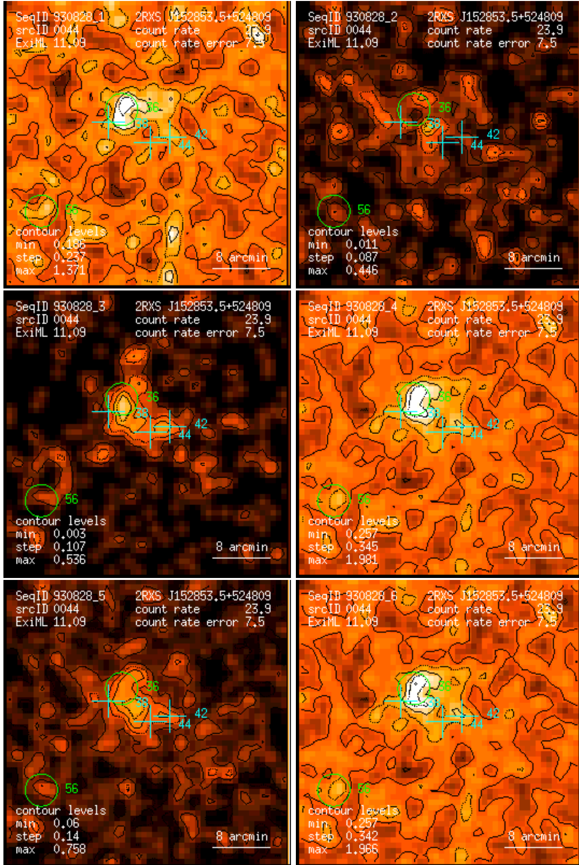
Figure 44: RASS 930828: detection 0044: band rate images, Gaussian filter: (1) PSPC channels 11 – 41, (2) 52 – 90, (3) 91 – 201, (4) 11 – 235, (5) 52 – 201, (6) 11 – 201. Broad band rates in counts/ks. Band rate contour levels in counts/ks/arcmin 2 .
