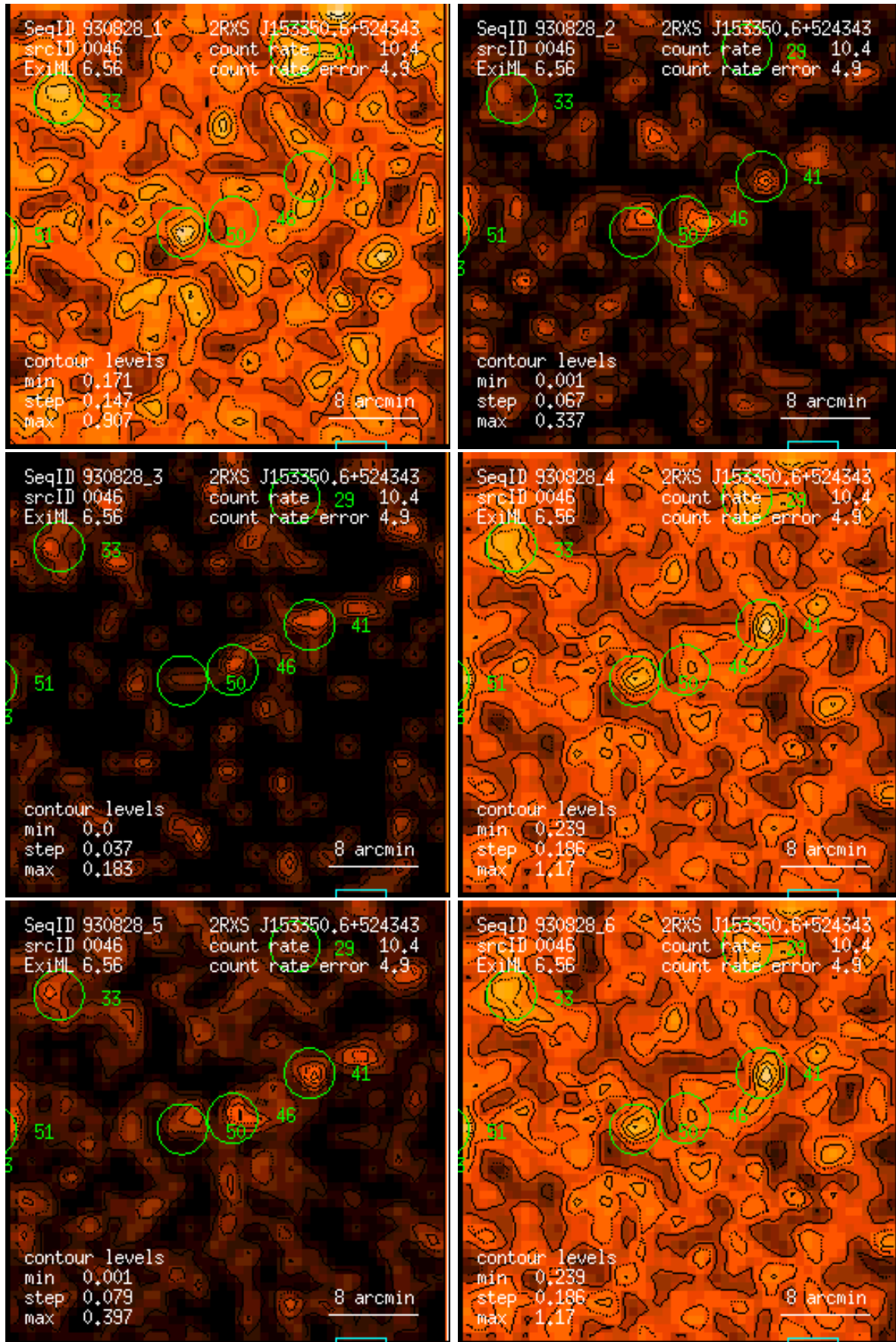
Figure 46: RASS 930828: detection 0046: band rate images, Gaussian filter: (1) PSPC channels 11 – 41, (2) 52 – 90, (3) 91 – 201, (4) 11 – 235, (5) 52 – 201, (6) 11 – 201. Broad band rates in counts/ks. Band rate contour levels in counts/ks/arcmin 2 .
