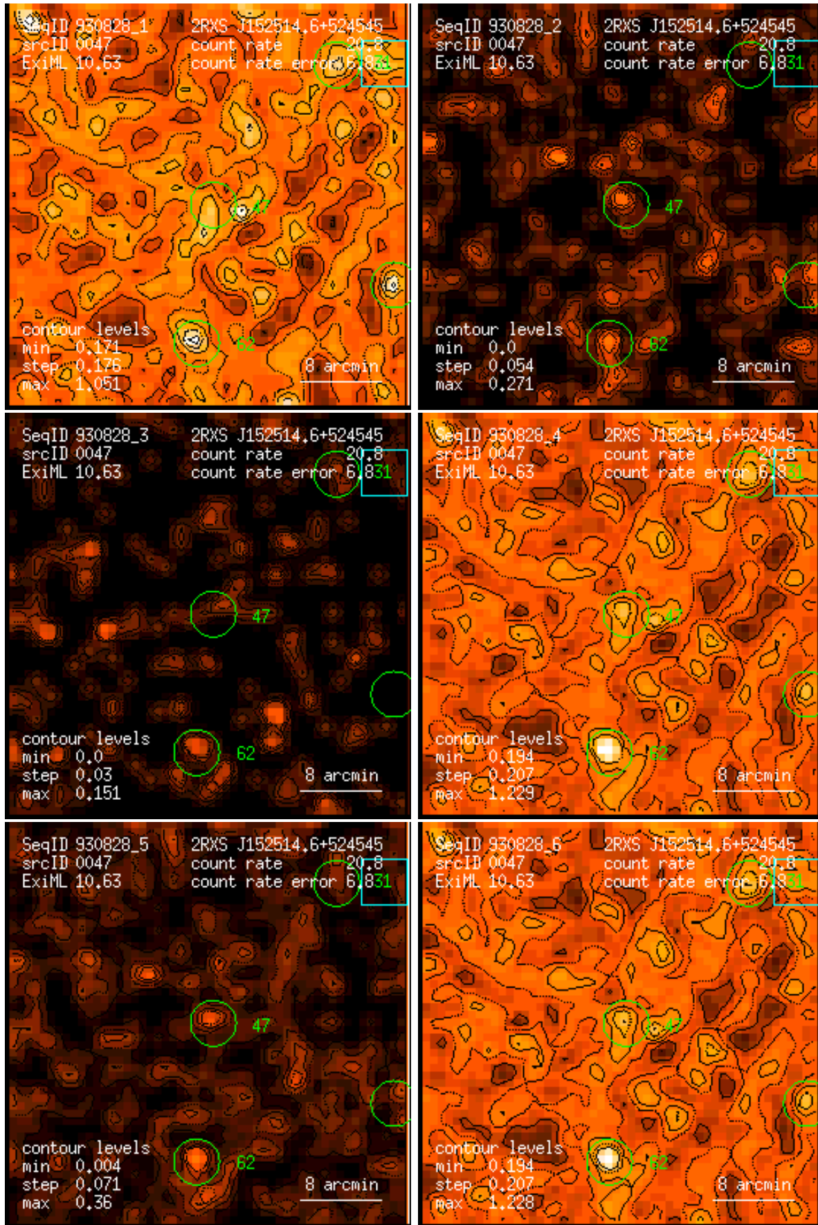
Figure 47: RASS 930828: detection 0047: band rate images, Gaussian filter: (1) PSPC channels 11 – 41, (2) 52 – 90, (3) 91 – 201, (4) 11 – 235, (5) 52 – 201, (6) 11 – 201. Broad band rates in counts/ks. Band rate contour levels in counts/ks/arcmin 2 .
