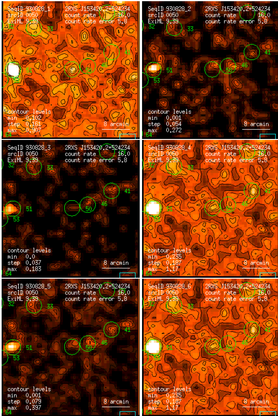
Figure 50: RASS 930828: detection 0050: band rate images, Gaussian filter: (1) PSPC channels 11 – 41, (2) 52 – 90, (3) 91 – 201, (4) 11 – 235, (5) 52 – 201, (6) 11 – 201. Broad band rates in counts/ks. Band rate contour levels in counts/ks/arcmin 2 .
