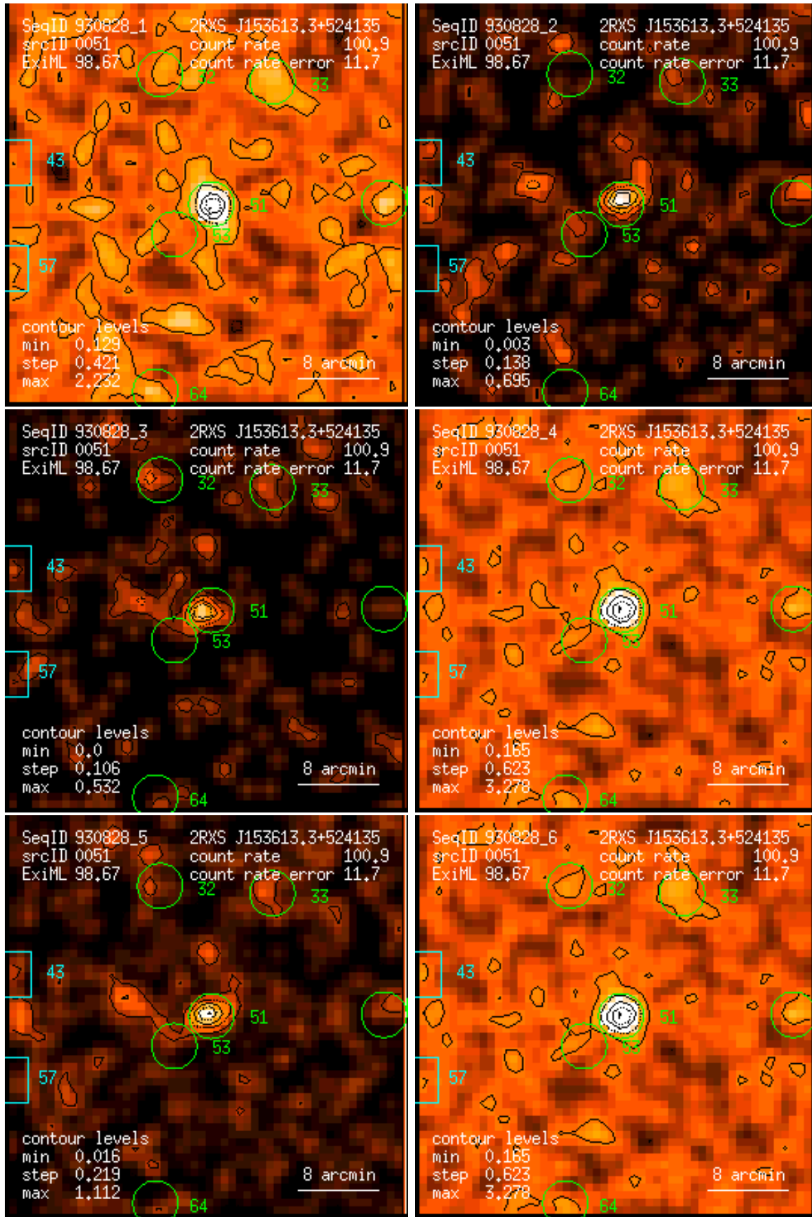
Figure 51: RASS 930828: detection 0051: band rate images, Gaussian filter: (1) PSPC channels 11 – 41, (2) 52 – 90, (3) 91 – 201, (4) 11 – 235, (5) 52 – 201, (6) 11 – 201. Broad band rates in counts/ks. Band rate contour levels in counts/ks/arcmin 2 .
