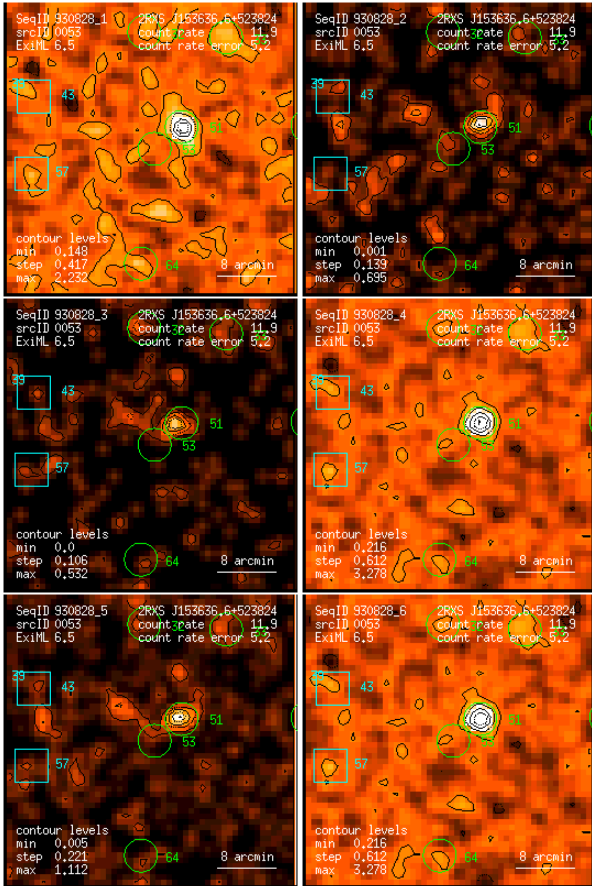
Figure 53: RASS 930828: detection 0053: band rate images, Gaussian filter: (1) PSPC channels 11 – 41, (2) 52 – 90, (3) 91 – 201, (4) 11 – 235, (5) 52 – 201, (6) 11 – 201. Broad band rates in counts/ks. Band rate contour levels in counts/ks/arcmin 2 .
