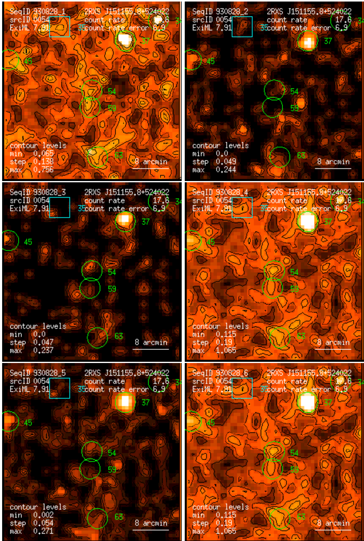
Figure 54: RASS 930828: detection 0054: band rate images, Gaussian filter: (1) PSPC channels 11 – 41, (2) 52 – 90, (3) 91 – 201, (4) 11 – 235, (5) 52 – 201, (6) 11 – 201. Broad band rates in counts/ks. Band rate contour levels in counts/ks/arcmin 2 .
