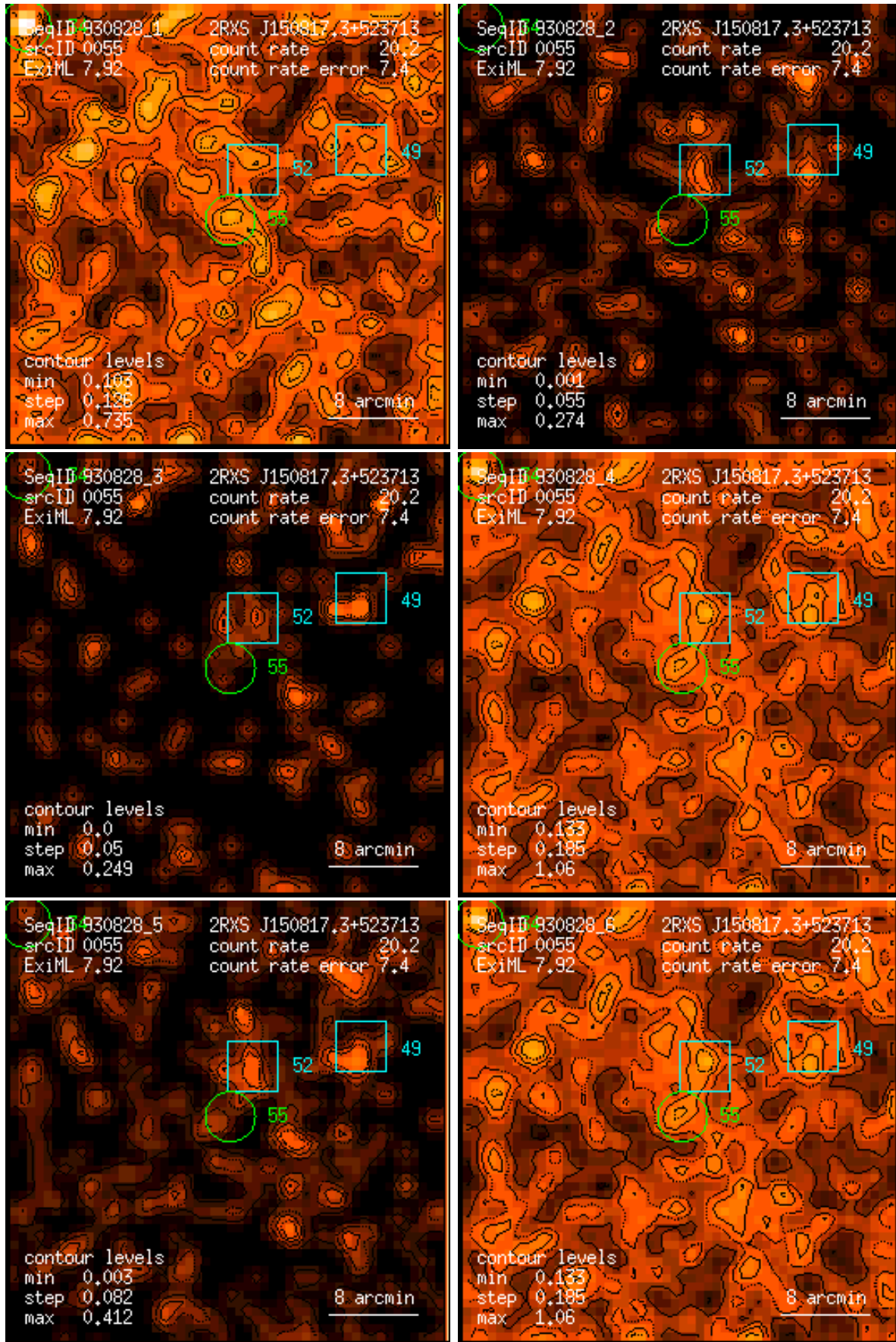
Figure 55: RASS 930828: detection 0055: band rate images, Gaussian filter: (1) PSPC channels 11 – 41, (2) 52 – 90, (3) 91 – 201, (4) 11 – 235, (5) 52 – 201, (6) 11 – 201. Broad band rates in counts/ks. Band rate contour levels in counts/ks/arcmin 2 .
