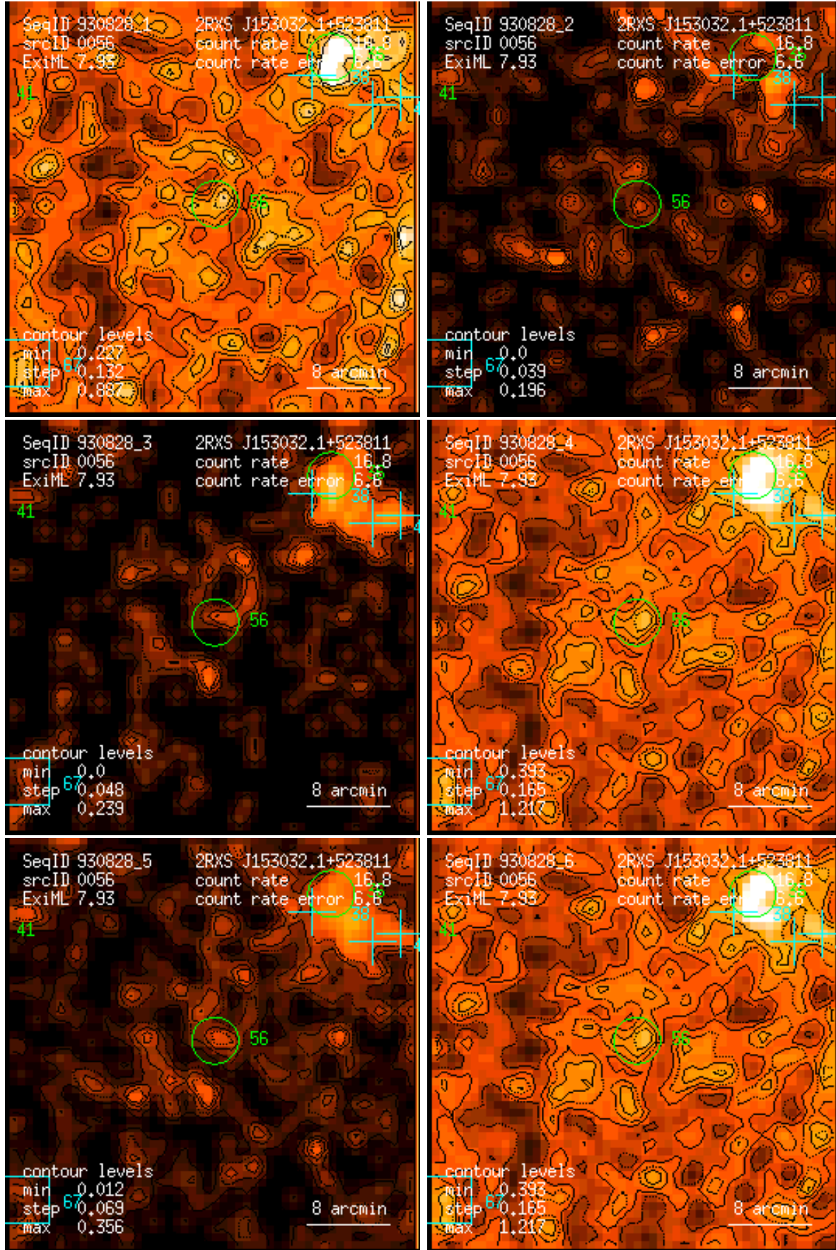
Figure 56: RASS 930828: detection 0056: band rate images, Gaussian filter: (1) PSPC channels 11 – 41, (2) 52 – 90, (3) 91 – 201, (4) 11 – 235, (5) 52 – 201, (6) 11 – 201. Broad band rates in counts/ks. Band rate contour levels in counts/ks/arcmin 2 .
