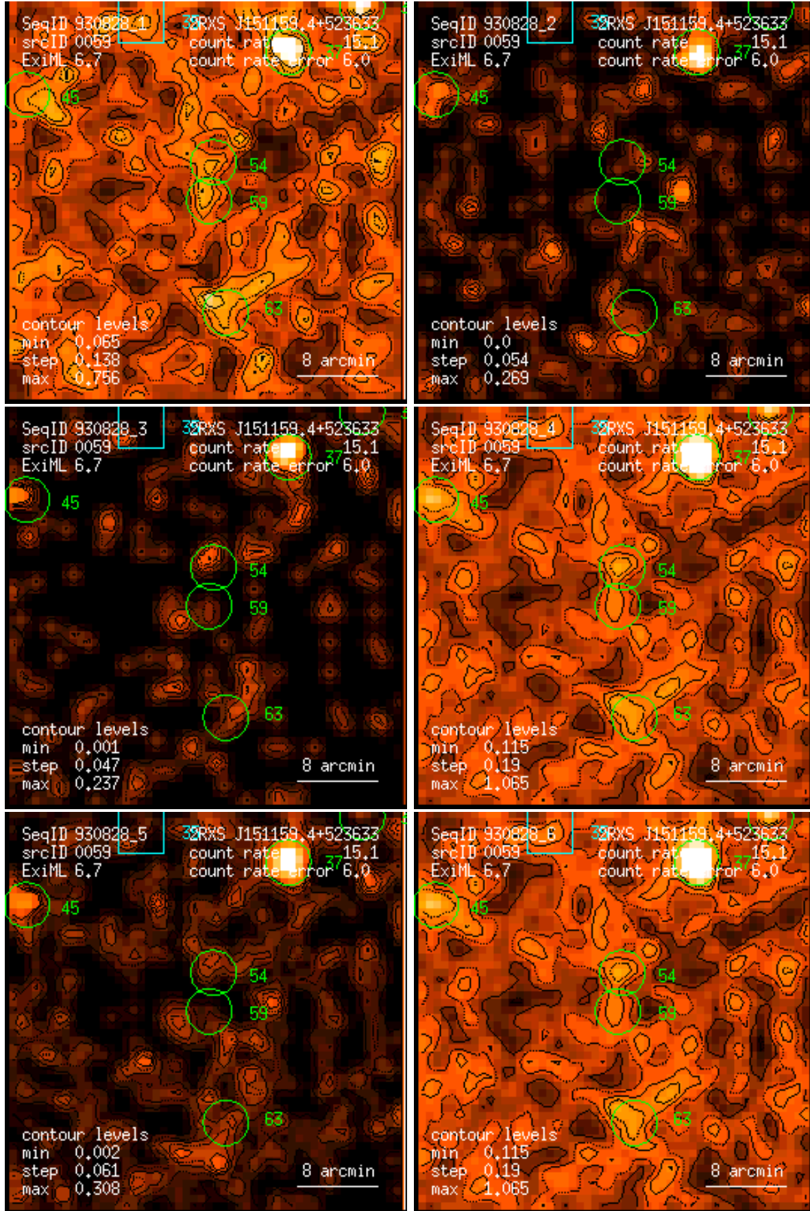
Figure 59: RASS 930828: detection 0059: band rate images, Gaussian filter: (1) PSPC channels 11 – 41, (2) 52 – 90, (3) 91 – 201, (4) 11 – 235, (5) 52 – 201, (6) 11 – 201. Broad band rates in counts/ks. Band rate contour levels in counts/ks/arcmin 2 .
