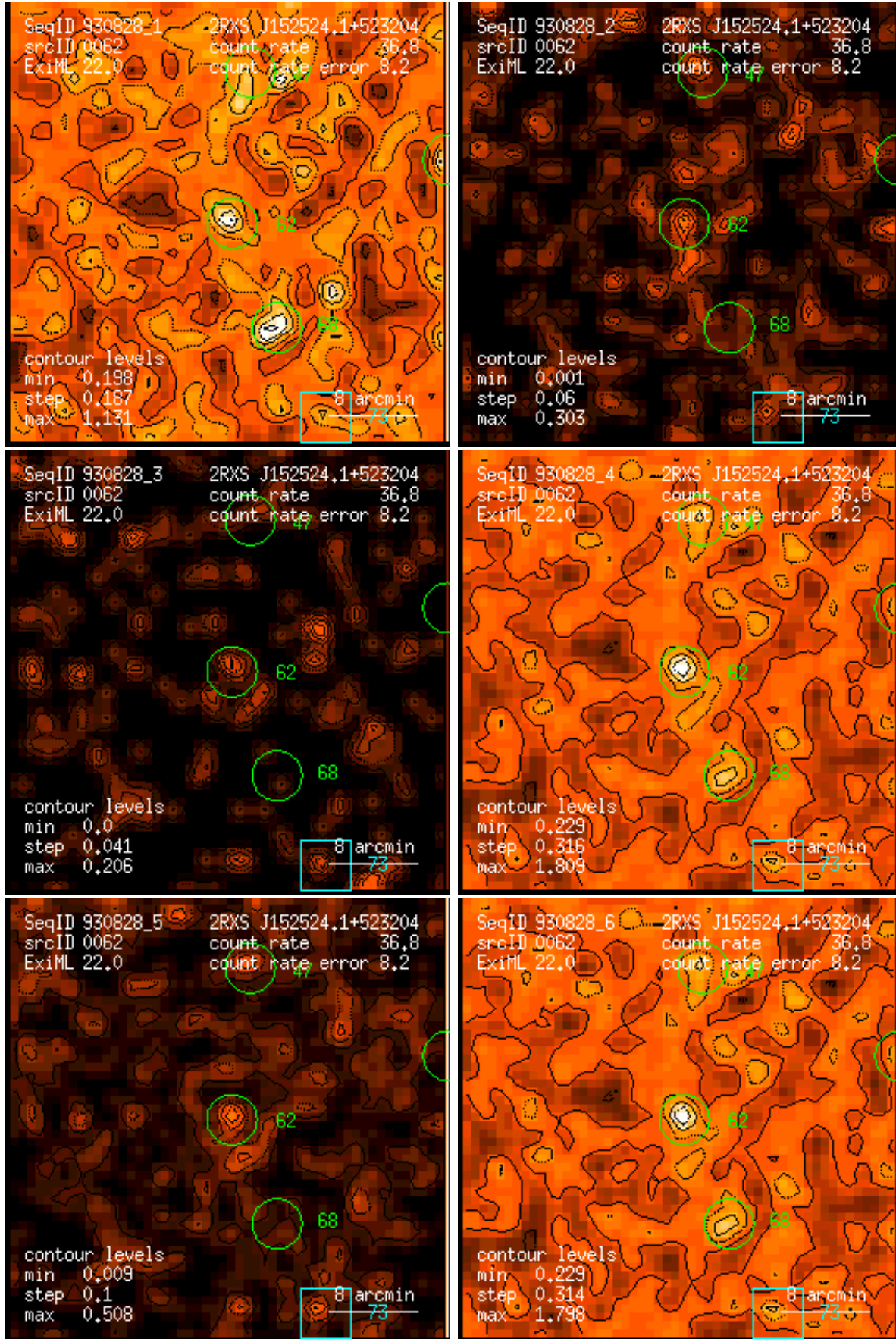
Figure 62: RASS 930828: detection 0062: band rate images, Gaussian filter: (1) PSPC channels 11 – 41, (2) 52 – 90, (3) 91 – 201, (4) 11 – 235, (5) 52 – 201, (6) 11 – 201. Broad band rates in counts/ks. Band rate contour levels in counts/ks/arcmin 2 .
