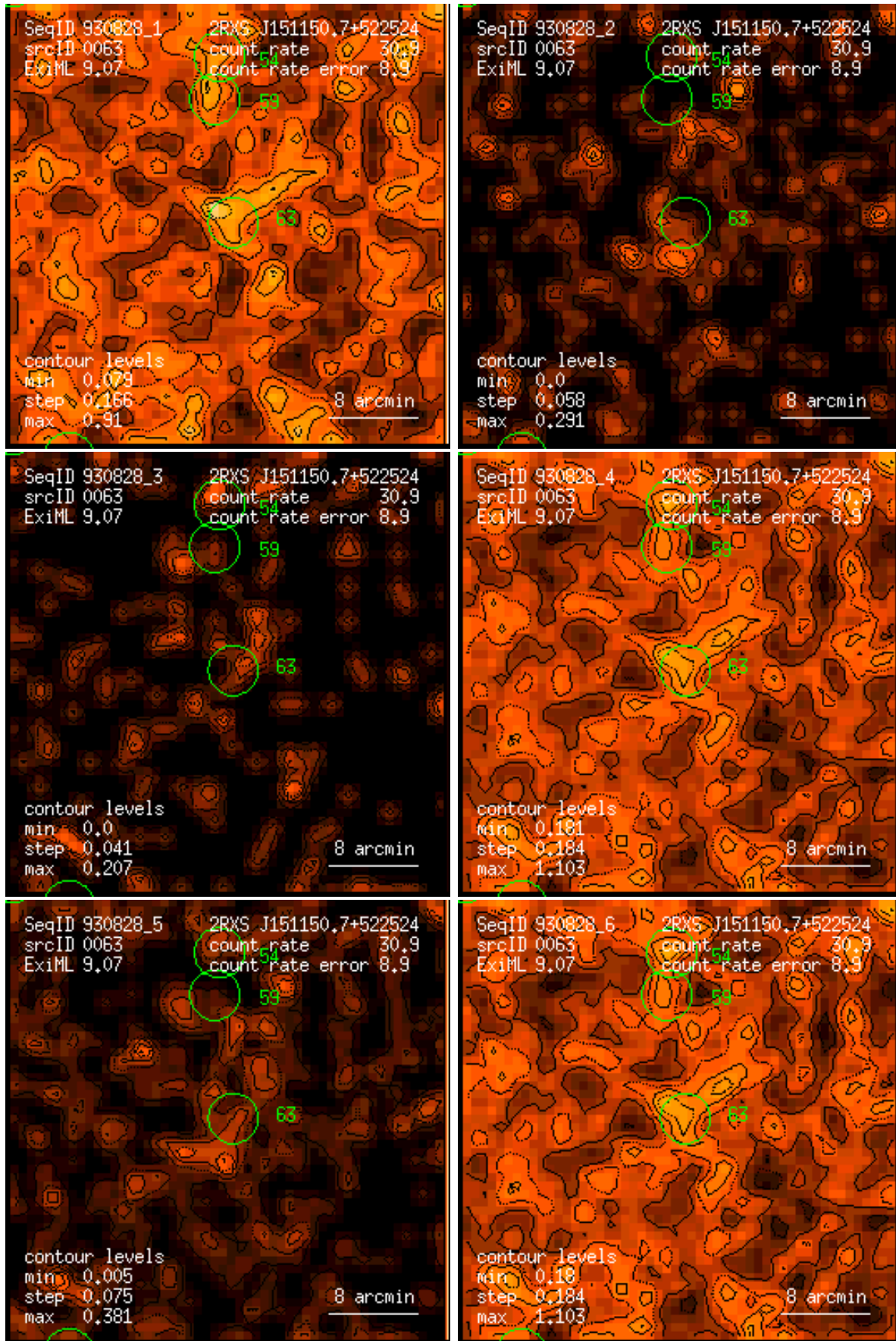
Figure 63: RASS 930828: detection 0063: band rate images, Gaussian filter: (1) PSPC channels 11 – 41, (2) 52 – 90, (3) 91 – 201, (4) 11 – 235, (5) 52 – 201, (6) 11 – 201. Broad band rates in counts/ks. Band rate contour levels in counts/ks/arcmin 2 .
