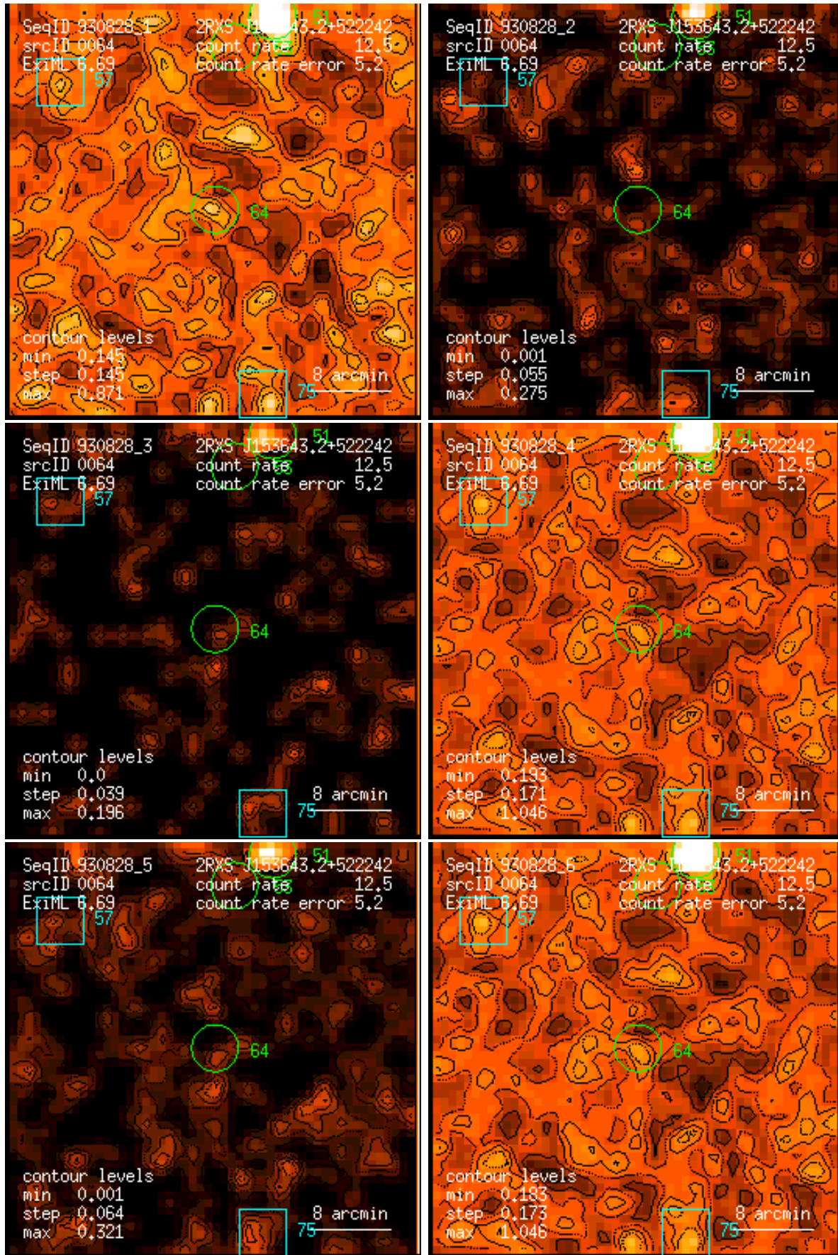
Figure 64: RASS 930828: detection 0064: band rate images, Gaussian filter: (1) PSPC channels 11 – 41, (2) 52 – 90, (3) 91 – 201, (4) 11 – 235, (5) 52 – 201, (6) 11 – 201. Broad band rates in counts/ks. Band rate contour levels in counts/ks/arcmin 2 .
