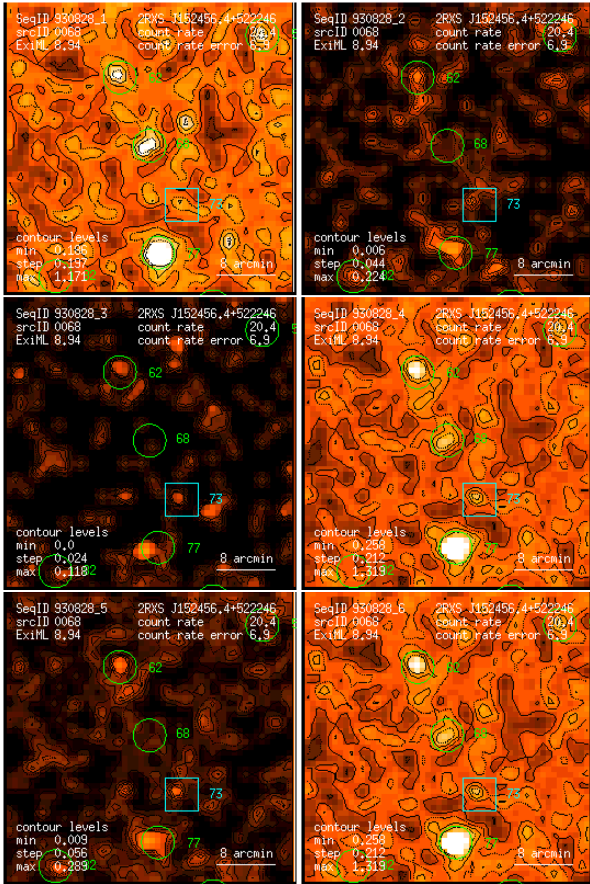
Figure 68: RASS 930828: detection 0068: band rate images, Gaussian filter: (1) PSPC channels 11 – 41, (2) 52 – 90, (3) 91 – 201, (4) 11 – 235, (5) 52 – 201, (6) 11 – 201. Broad band rates in counts/ks. Band rate contour levels in counts/ks/arcmin 2 .
