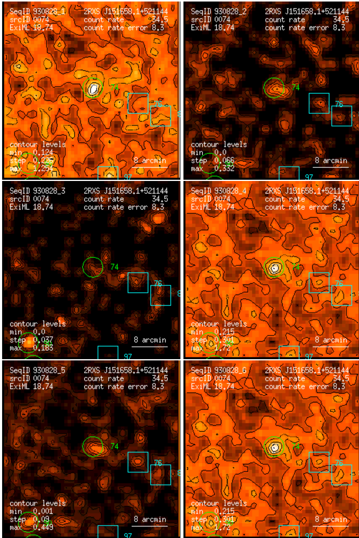
Figure 74: RASS 930828: detection 0074: band rate images, Gaussian filter: (1) PSPC channels 11 – 41, (2) 52 – 90, (3) 91 – 201, (4) 11 – 235, (5) 52 – 201, (6) 11 – 201. Broad band rates in counts/ks. Band rate contour levels in counts/ks/arcmin 2 .
