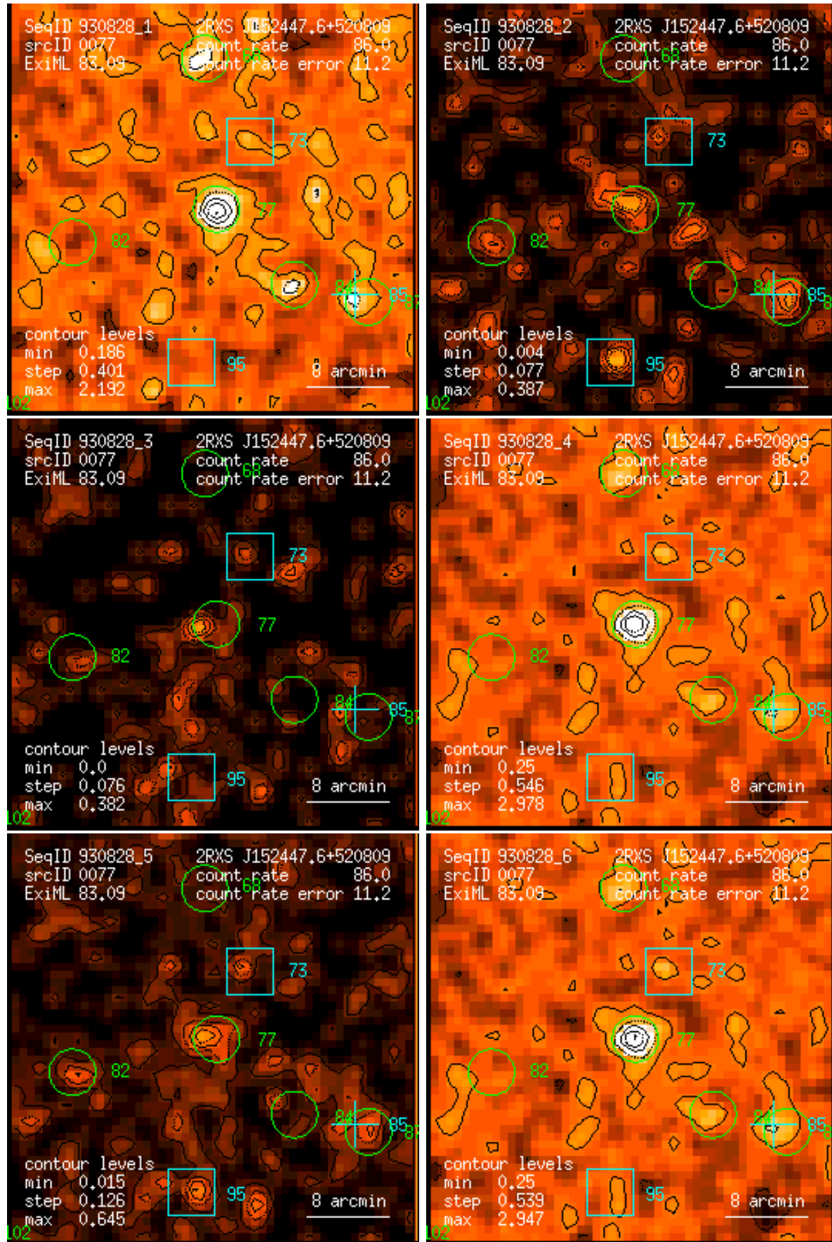
Figure 77: RASS 930828: detection 0077: band rate images, Gaussian filter: (1) PSPC channels 11 – 41, (2) 52 – 90, (3) 91 – 201, (4) 11 – 235, (5) 52 – 201, (6) 11 – 201. Broad band rates in counts/ks. Band rate contour levels in counts/ks/arcmin 2 .
