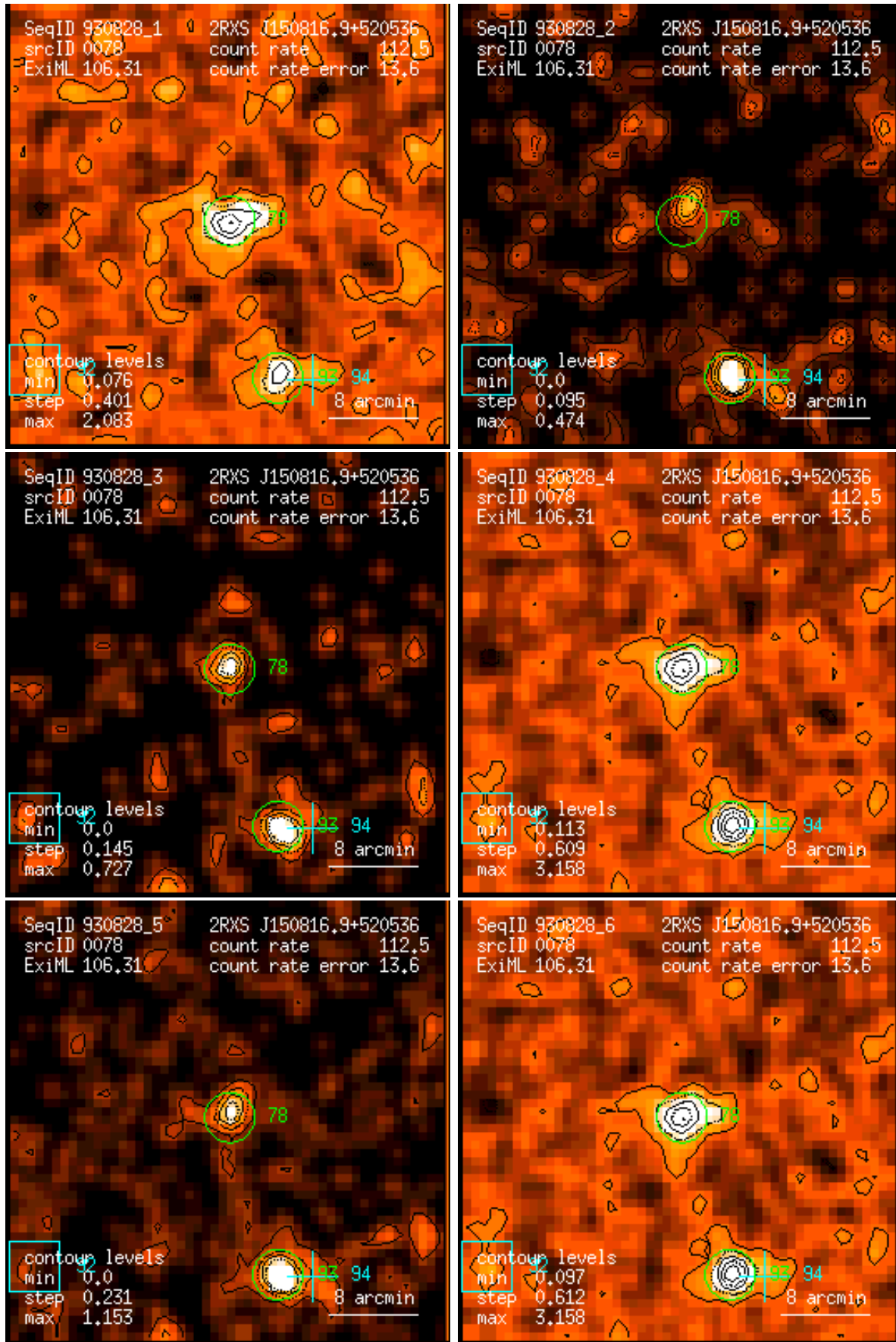
Figure 78: RASS 930828: detection 0078: band rate images, Gaussian filter: (1) PSPC channels 11 – 41, (2) 52 – 90, (3) 91 – 201, (4) 11 – 235, (5) 52 – 201, (6) 11 – 201. Broad band rates in counts/ks. Band rate contour levels in counts/ks/arcmin 2 .
