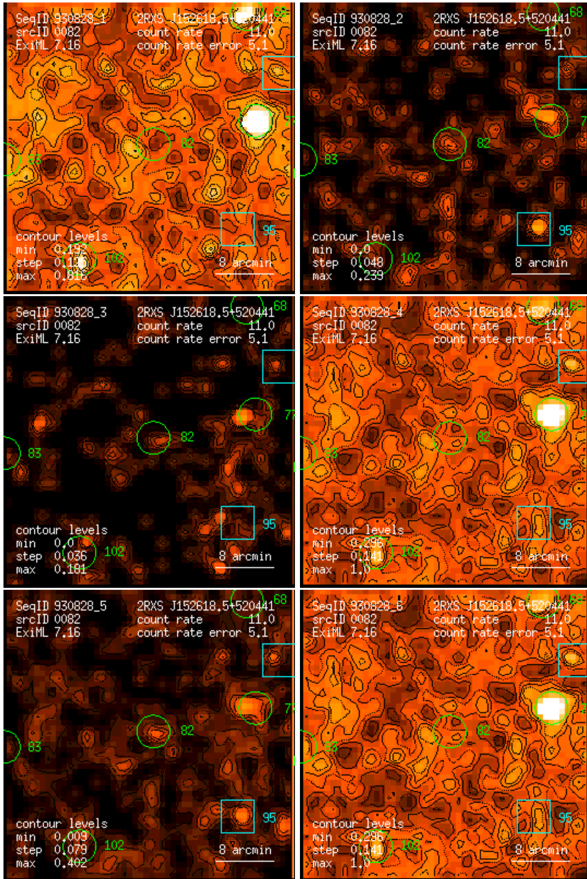
Figure 82: RASS 930828: detection 0082: band rate images, Gaussian filter: (1) PSPC channels 11 – 41, (2) 52 – 90, (3) 91 – 201, (4) 11 – 235, (5) 52 – 201, (6) 11 – 201. Broad band rates in counts/ks. Band rate contour levels in counts/ks/arcmin 2 .
