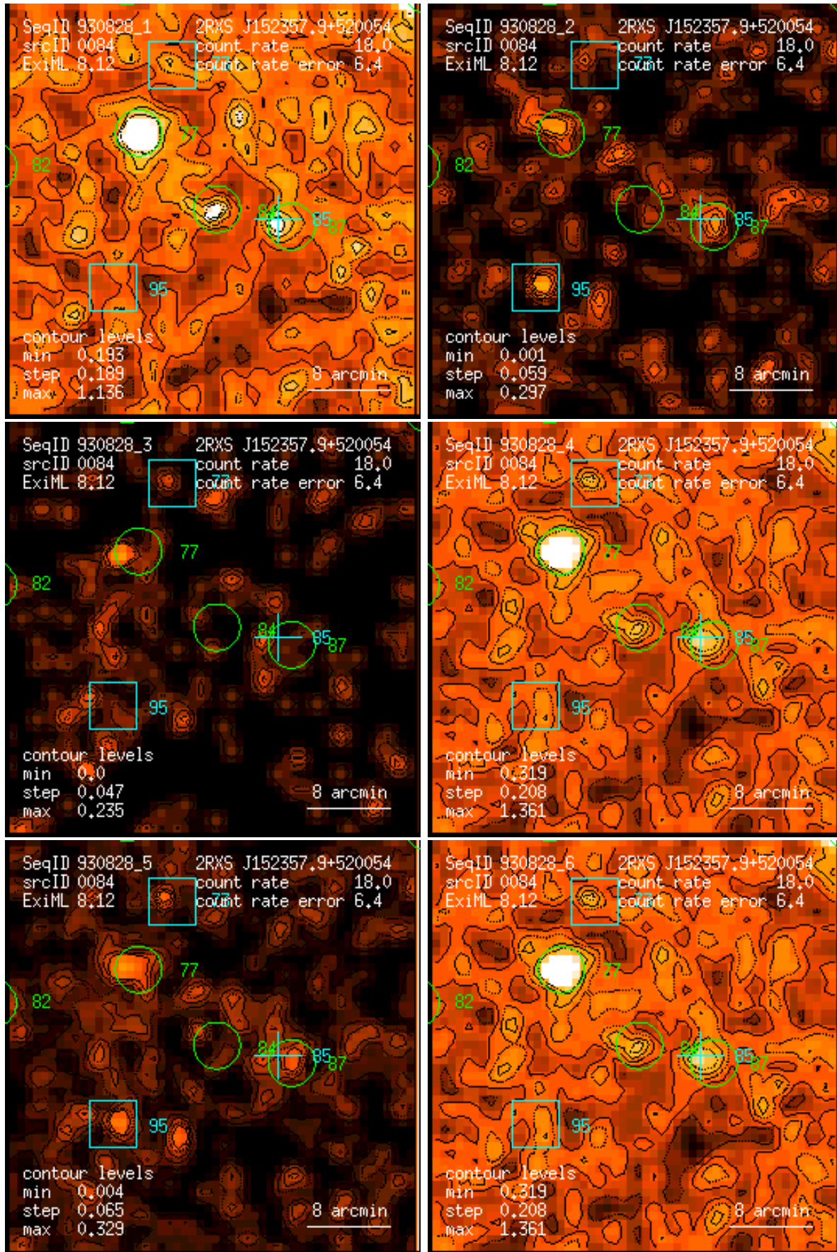
Figure 84: RASS 930828: detection 0084: band rate images, Gaussian filter: (1) PSPC channels 11 – 41, (2) 52 – 90, (3) 91 – 201, (4) 11 – 235, (5) 52 – 201, (6) 11 – 201. Broad band rates in counts/ks. Band rate contour levels in counts/ks/arcmin 2 .
