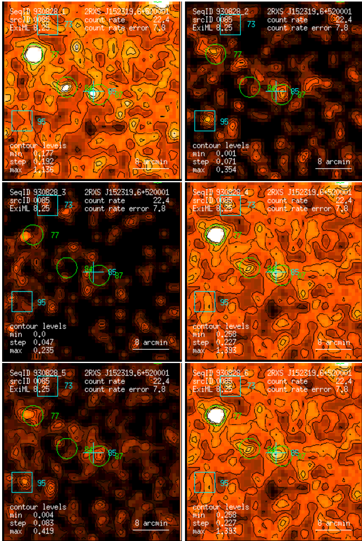
Figure 85: RASS 930828: detection 0085: band rate images, Gaussian filter: (1) PSPC channels 11 – 41, (2) 52 – 90, (3) 91 – 201, (4) 11 – 235, (5) 52 – 201, (6) 11 – 201. Broad band rates in counts/ks. Band rate contour levels in counts/ks/arcmin 2 .
