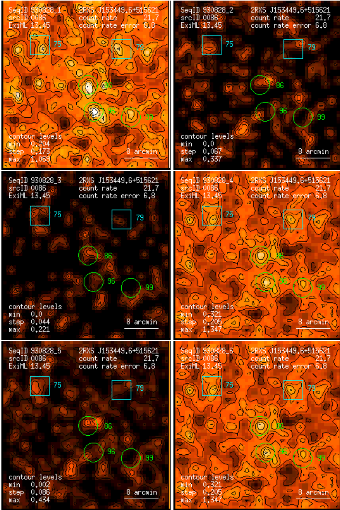
Figure 86: RASS 930828: detection 0086: band rate images, Gaussian filter: (1) PSPC channels 11 – 41, (2) 52 – 90, (3) 91 – 201, (4) 11 – 235, (5) 52 – 201, (6) 11 – 201. Broad band rates in counts/ks. Band rate contour levels in counts/ks/arcmin 2 .
