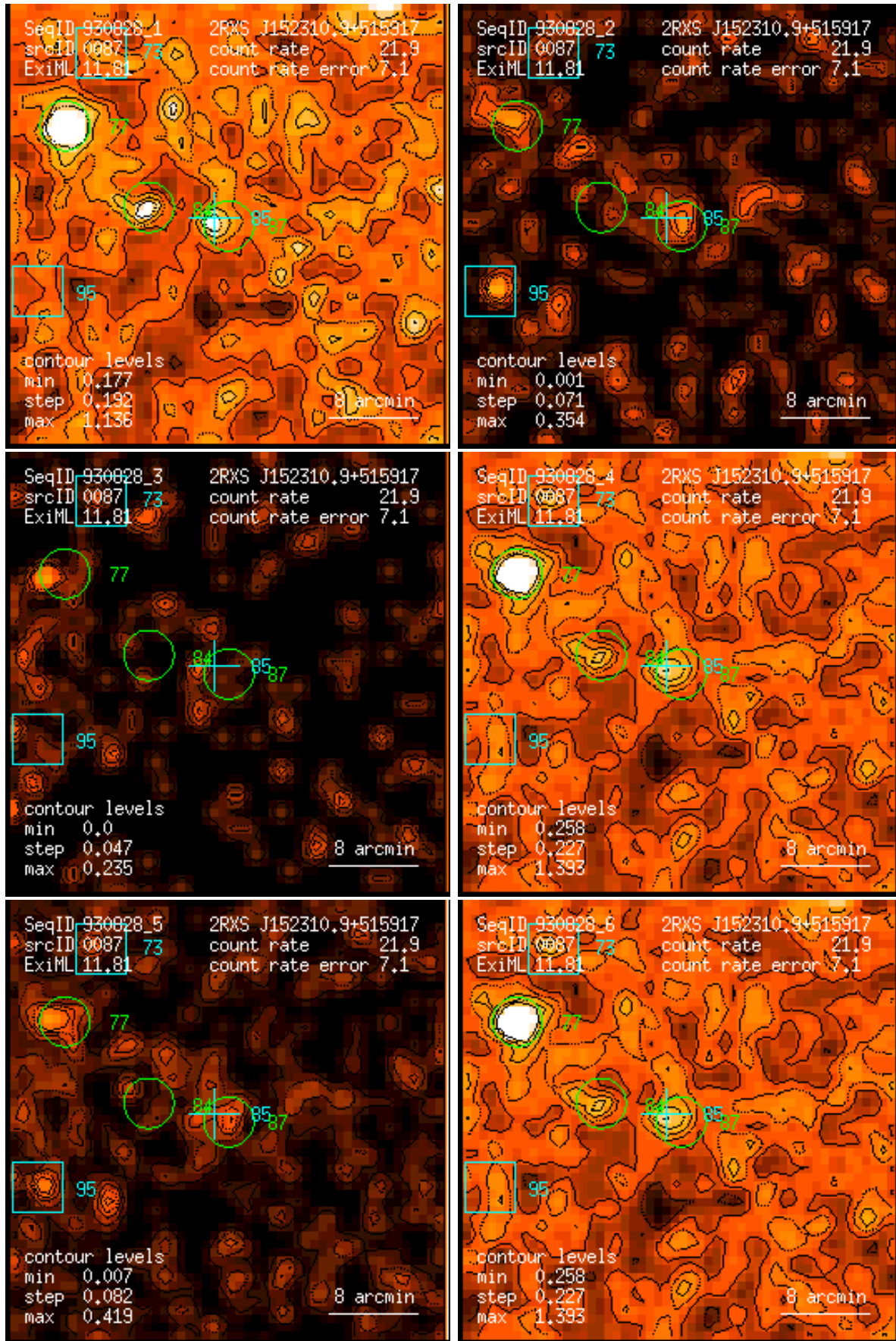
Figure 87: RASS 930828: detection 0087: band rate images, Gaussian filter: (1) PSPC channels 11 – 41, (2) 52 – 90, (3) 91 – 201, (4) 11 – 235, (5) 52 – 201, (6) 11 – 201. Broad band rates in counts/ks. Band rate contour levels in counts/ks/arcmin 2 .
