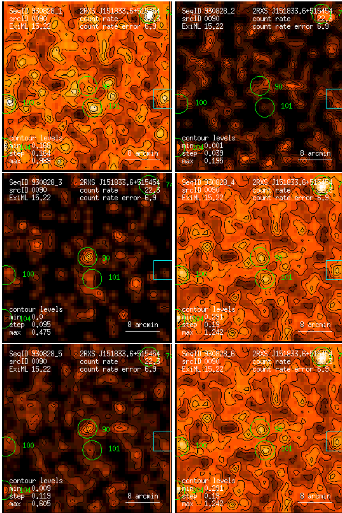
Figure 90: RASS 930828: detection 0090: band rate images, Gaussian filter: (1) PSPC channels 11 – 41, (2) 52 – 90, (3) 91 – 201, (4) 11 – 235, (5) 52 – 201, (6) 11 – 201. Broad band rates in counts/ks. Band rate contour levels in counts/ks/arcmin 2 .
