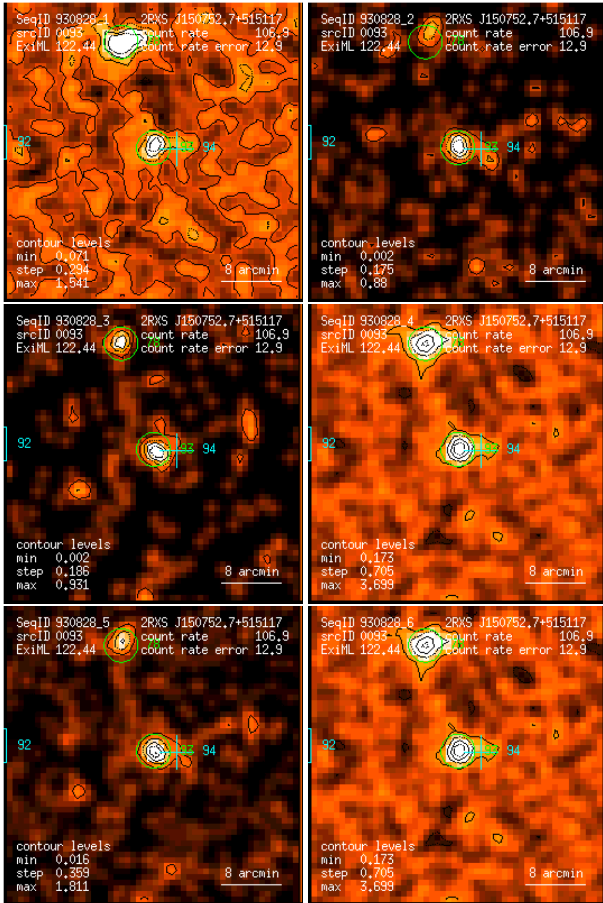
Figure 93: RASS 930828: detection 0093: band rate images, Gaussian filter: (1) PSPC channels 11 – 41, (2) 52 – 90, (3) 91 – 201, (4) 11 – 235, (5) 52 – 201, (6) 11 – 201. Broad band rates in counts/ks. Band rate contour levels in counts/ks/arcmin 2 .
