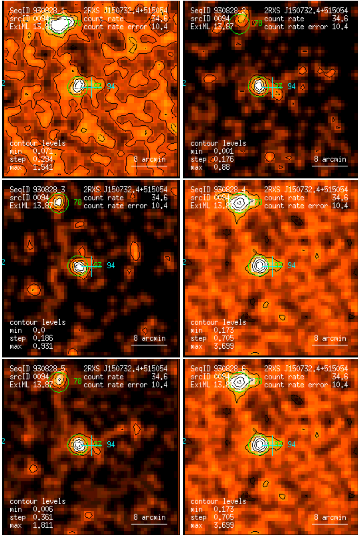
Figure 94: RASS 930828: detection 0094: band rate images, Gaussian filter: (1) PSPC channels 11 – 41, (2) 52 – 90, (3) 91 – 201, (4) 11 – 235, (5) 52 – 201, (6) 11 – 201. Broad band rates in counts/ks. Band rate contour levels in counts/ks/arcmin 2 .
