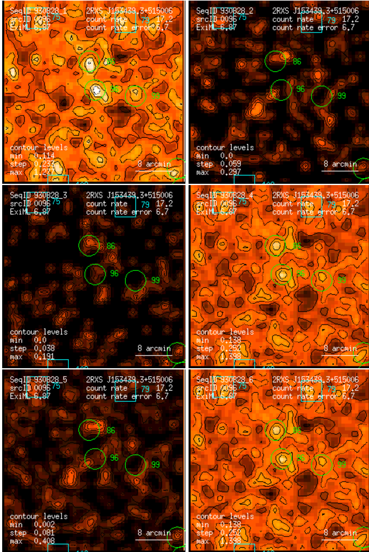
Figure 96: RASS 930828: detection 0096: band rate images, Gaussian filter: (1) PSPC channels 11 – 41, (2) 52 – 90, (3) 91 – 201, (4) 11 – 235, (5) 52 – 201, (6) 11 – 201. Broad band rates in counts/ks. Band rate contour levels in counts/ks/arcmin 2 .
