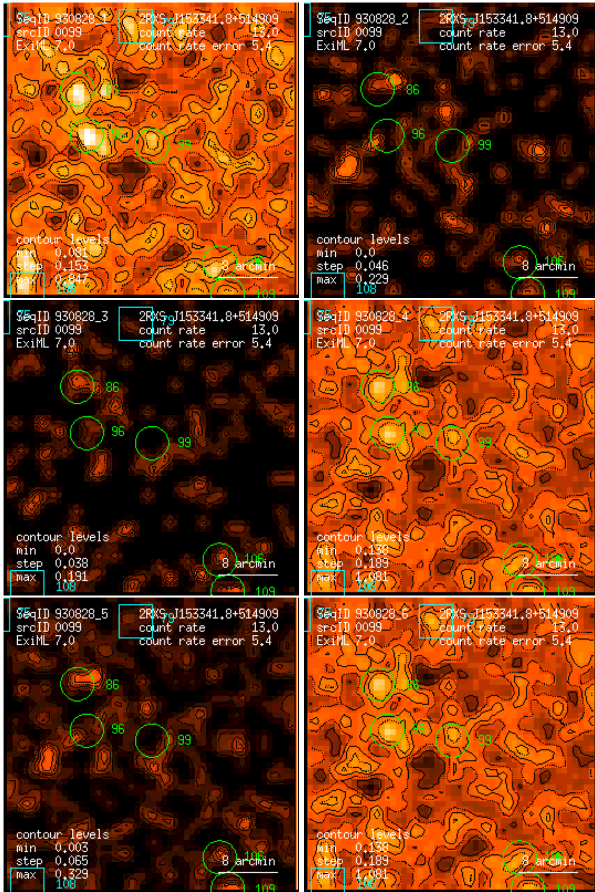
Figure 99: RASS 930828: detection 0099: band rate images, Gaussian filter: (1) PSPC channels 11 – 41, (2) 52 – 90, (3) 91 – 201, (4) 11 – 235, (5) 52 – 201, (6) 11 – 201. Broad band rates in counts/ks. Band rate contour levels in counts/ks/arcmin 2 .
