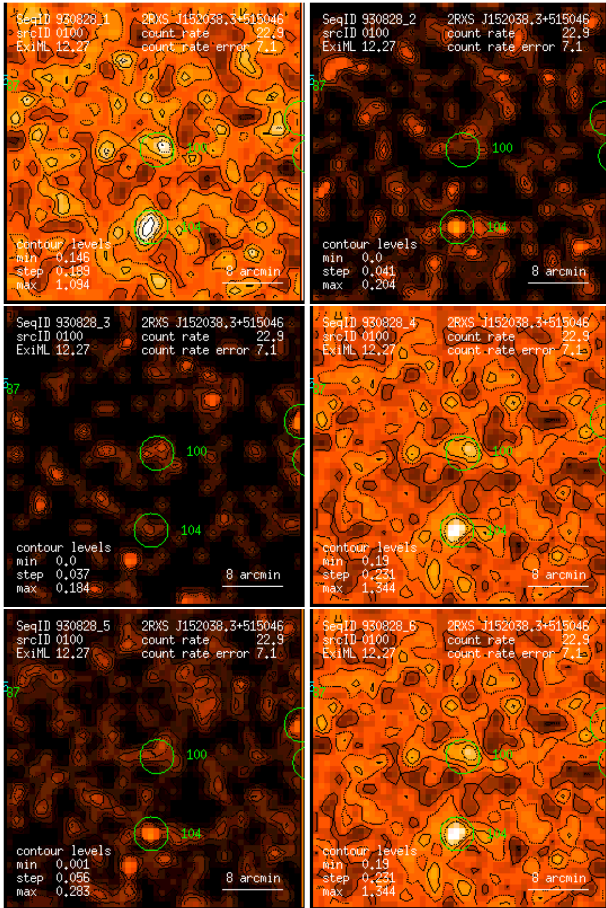
Figure 100: RASS 930828: detection 0100: band rate images, Gaussian filter: (1) PSPC channels 11 – 41, (2) 52 – 90, (3) 91 – 201, (4) 11 – 235, (5) 52 – 201, (6) 11 – 201. Broad band rates in counts/ks. Band rate contour levels in counts/ks/arcmin 2 .
