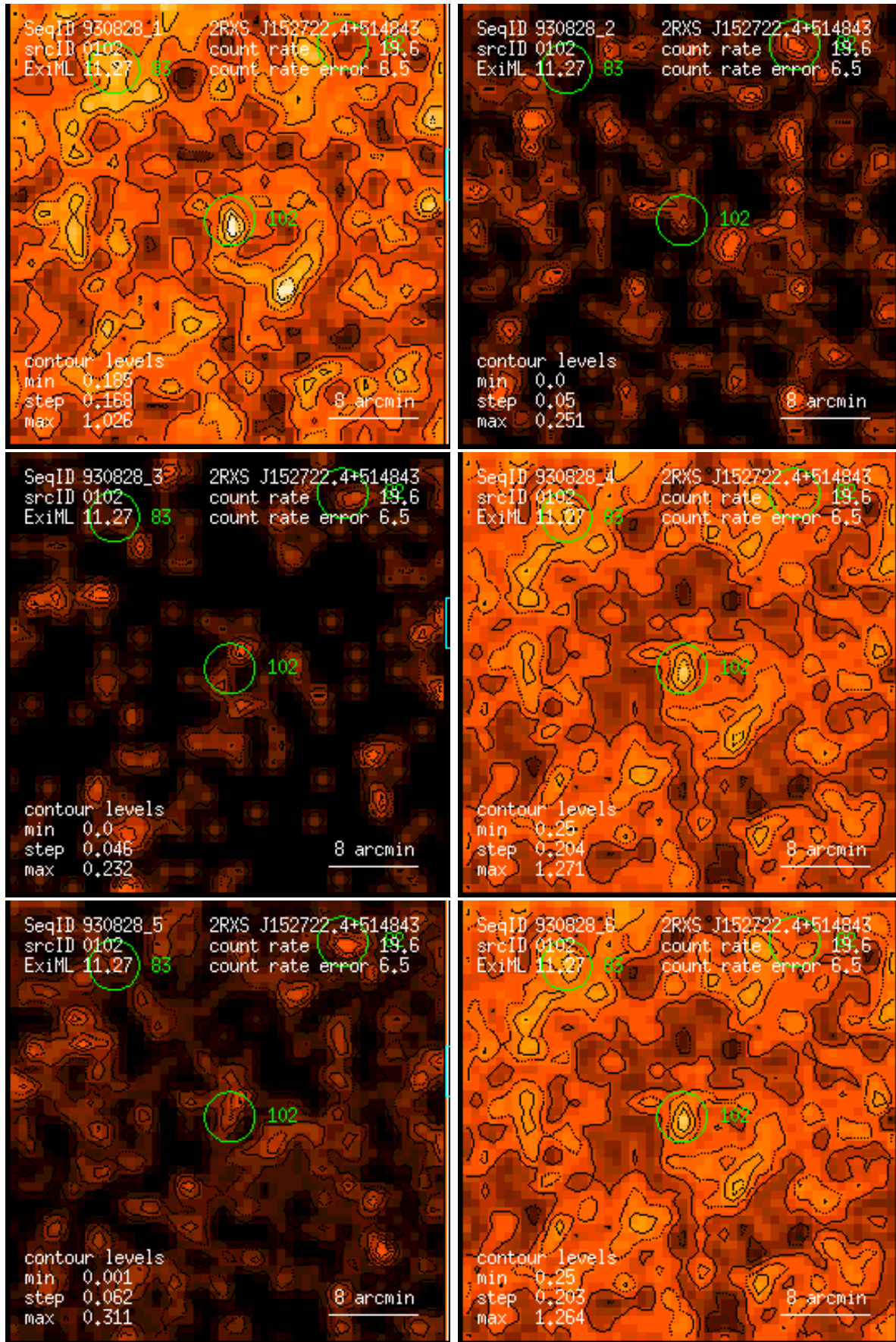
Figure 102: RASS 930828: detection 0102: band rate images, Gaussian filter: (1) PSPC channels 11 – 41, (2) 52 – 90, (3) 91 – 201, (4) 11 – 235, (5) 52 – 201, (6) 11 – 201. Broad band rates in counts/ks. Band rate contour levels in counts/ks/arcmin 2 .
