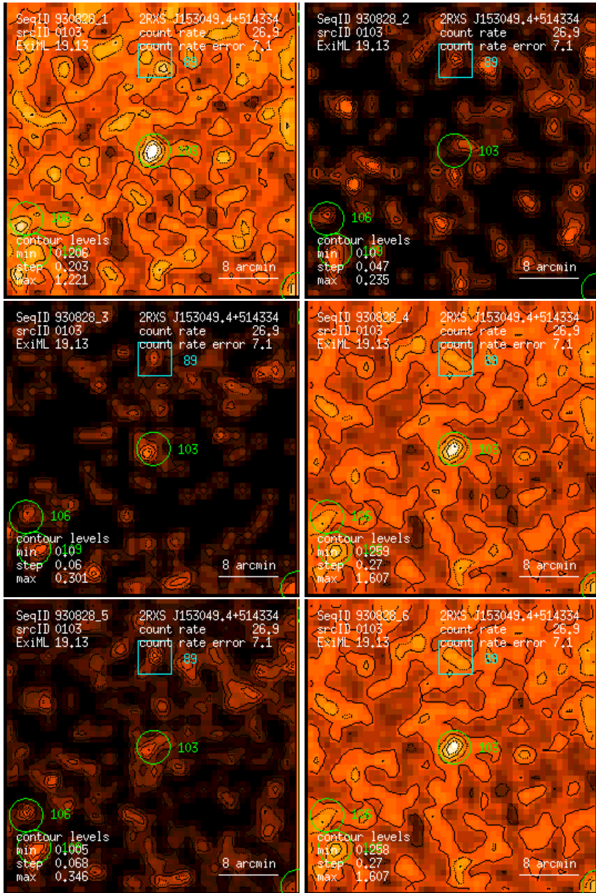
Figure 103: RASS 930828: detection 0103: band rate images, Gaussian filter: (1) PSPC channels 11 – 41, (2) 52 – 90, (3) 91 – 201, (4) 11 – 235, (5) 52 – 201, (6) 11 – 201. Broad band rates in counts/ks. Band rate contour levels in counts/ks/arcmin 2 .
