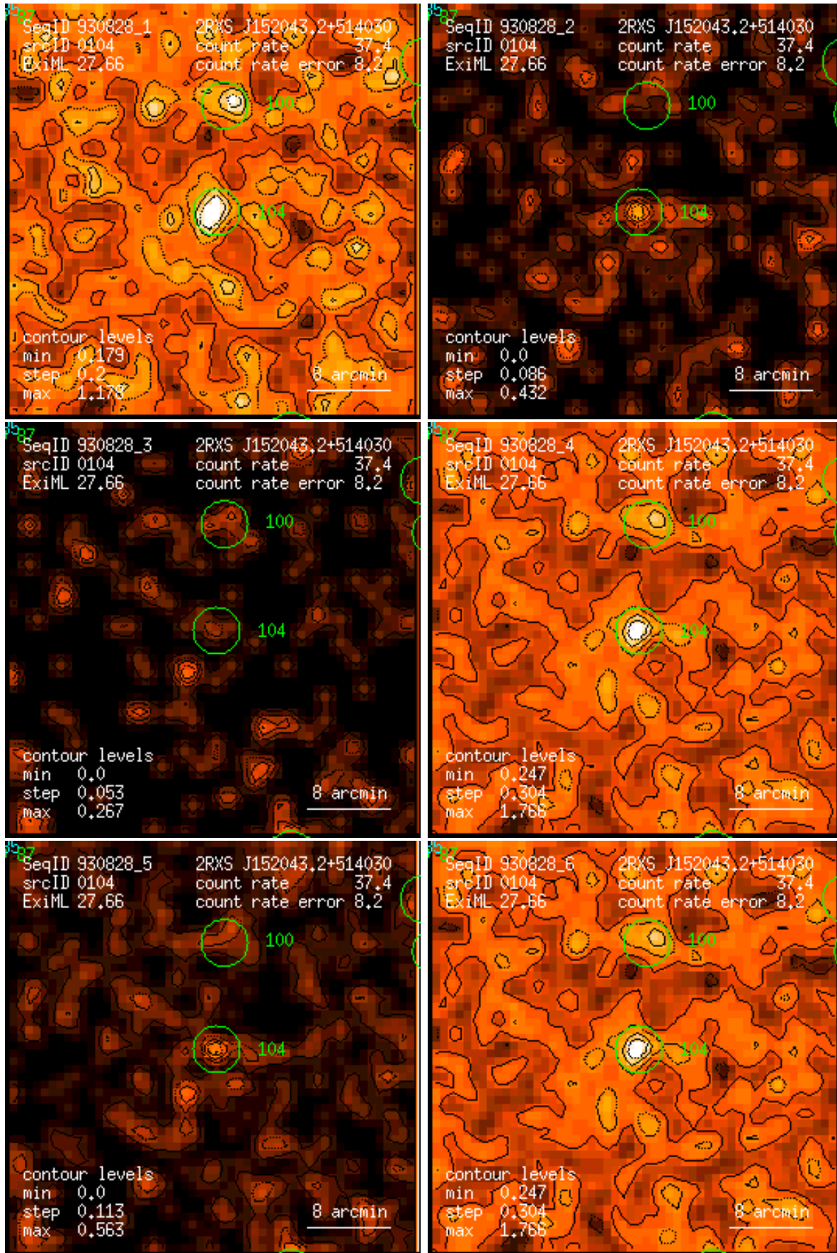
Figure 104: RASS 930828: detection 0104: band rate images, Gaussian filter: (1) PSPC channels 11 – 41, (2) 52 – 90, (3) 91 – 201, (4) 11 – 235, (5) 52 – 201, (6) 11 – 201. Broad band rates in counts/ks. Band rate contour levels in counts/ks/arcmin 2 .
