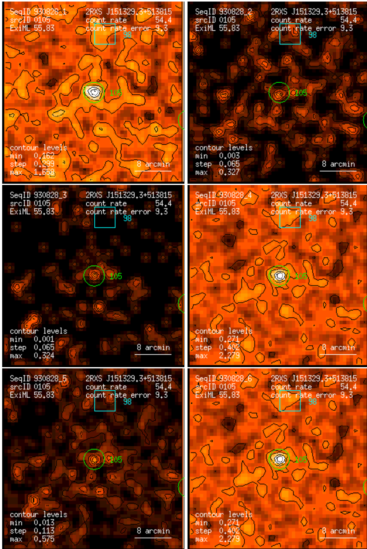
Figure 105: RASS 930828: detection 0105: band rate images, Gaussian filter: (1) PSPC channels 11 – 41, (2) 52 – 90, (3) 91 – 201, (4) 11 – 235, (5) 52 – 201, (6) 11 – 201. Broad band rates in counts/ks. Band rate contour levels in counts/ks/arcmin 2 .
