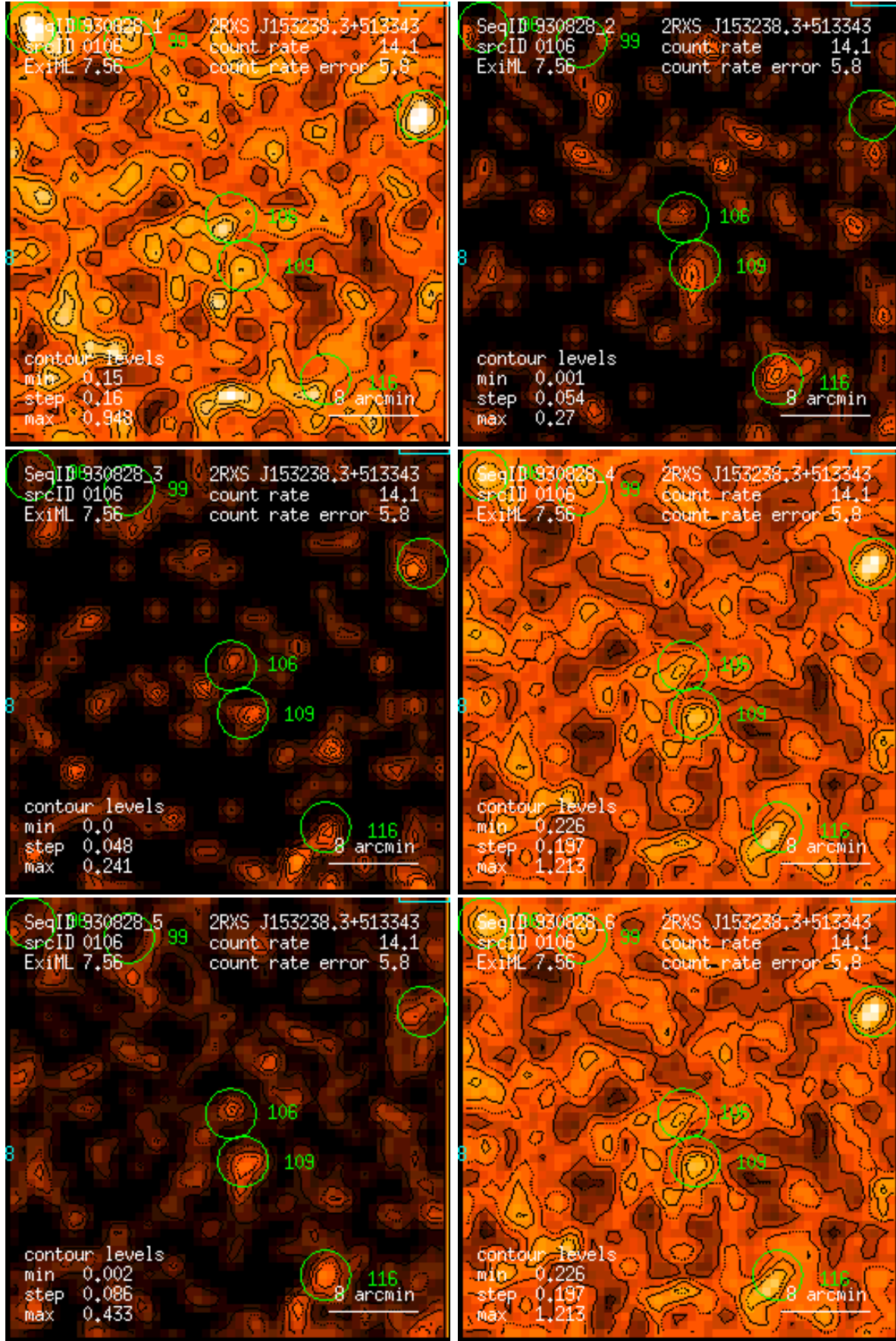
Figure 106: RASS 930828: detection 0106: band rate images, Gaussian filter: (1) PSPC channels 11 – 41, (2) 52 – 90, (3) 91 – 201, (4) 11 – 235, (5) 52 – 201, (6) 11 – 201. Broad band rates in counts/ks. Band rate contour levels in counts/ks/arcmin 2 .
