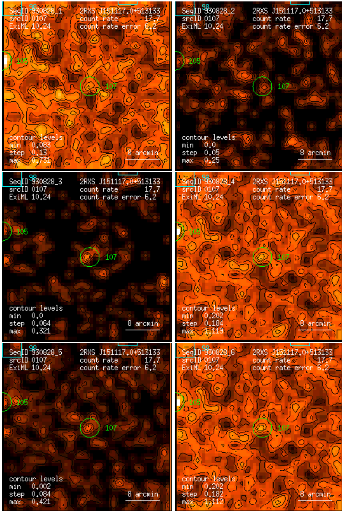
Figure 107: RASS 930828: detection 0107: band rate images, Gaussian filter: (1) PSPC channels 11 – 41, (2) 52 – 90, (3) 91 – 201, (4) 11 – 235, (5) 52 – 201, (6) 11 – 201. Broad band rates in counts/ks. Band rate contour levels in counts/ks/arcmin 2 .
