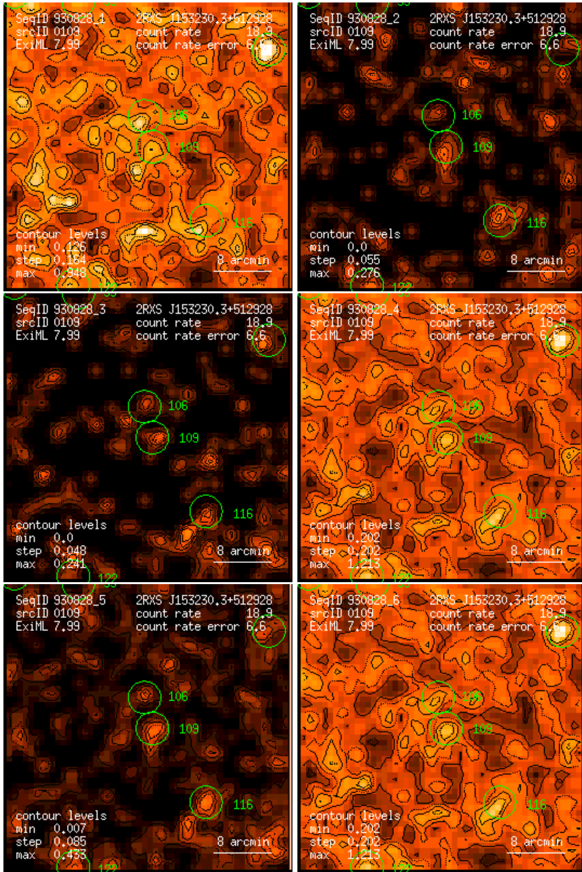
Figure 109: RASS 930828: detection 0109: band rate images, Gaussian filter: (1) PSPC channels 11 – 41, (2) 52 – 90, (3) 91 – 201, (4) 11 – 235, (5) 52 – 201, (6) 11 – 201. Broad band rates in counts/ks. Band rate contour levels in counts/ks/arcmin 2 .
