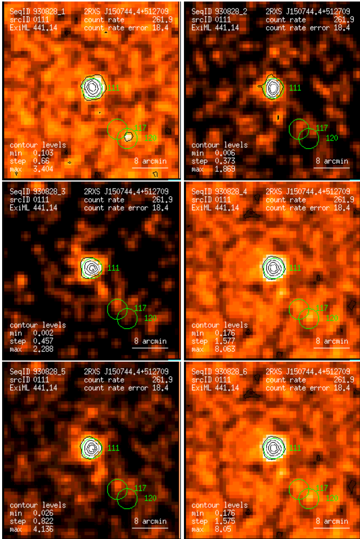
Figure 111: RASS 930828: detection 0111: band rate images, Gaussian filter: (1) PSPC channels 11 – 41, (2) 52 – 90, (3) 91 – 201, (4) 11 – 235, (5) 52 – 201, (6) 11 – 201. Broad band rates in counts/ks. Band rate contour levels in counts/ks/arcmin 2 .
