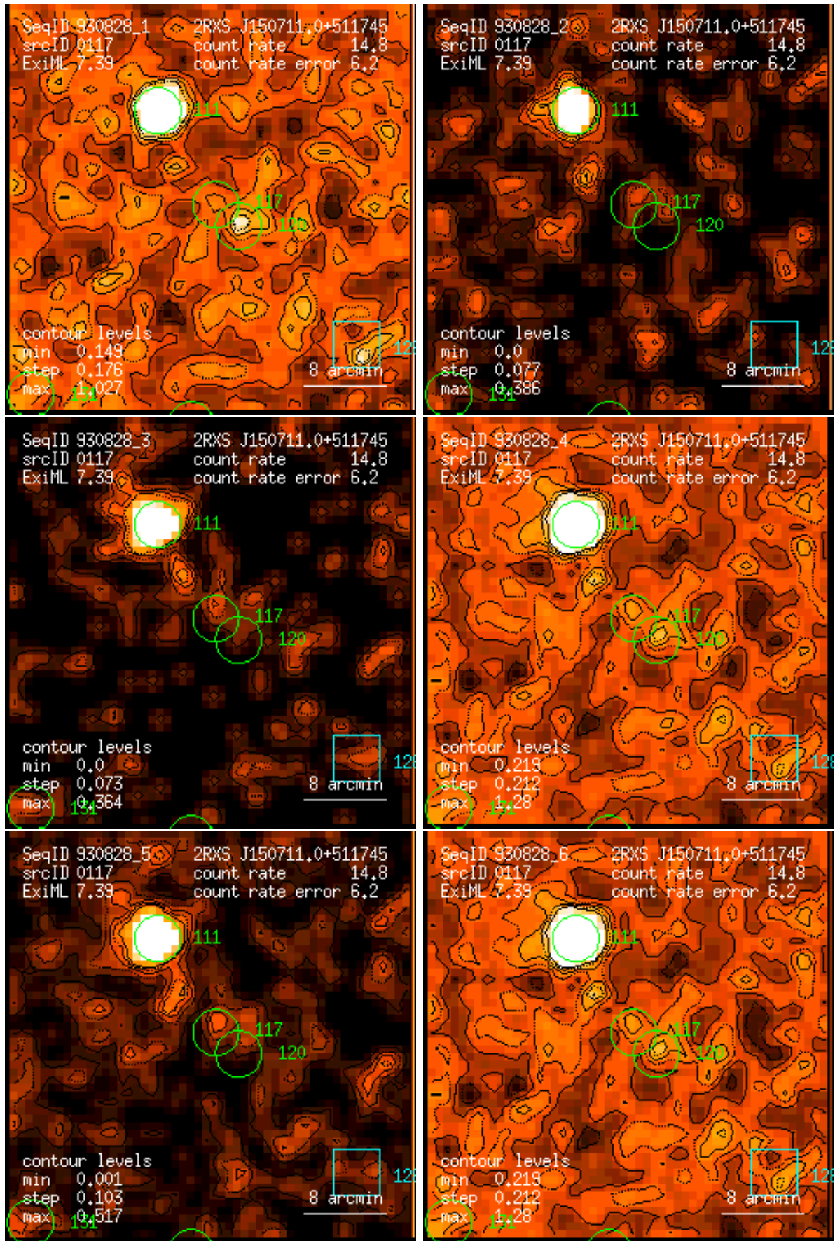
Figure 117: RASS 930828: detection 0117: band rate images, Gaussian filter: (1) PSPC channels 11 – 41, (2) 52 – 90, (3) 91 – 201, (4) 11 – 235, (5) 52 – 201, (6) 11 – 201. Broad band rates in counts/ks. Band rate contour levels in counts/ks/arcmin 2 .
